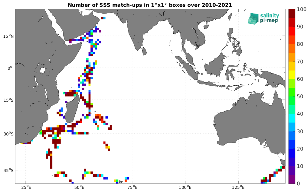
Figure 5: Number of SSS match-ups between TSG (GOSUD-Research-vessel) SSS and the SMOS SSS L2Q v333 - 0.25 Deg (CATDS-CPDC) SSS product for the Indian Ocean Pi-MEP region over 1°×1° boxes and for the full satellite product period.
