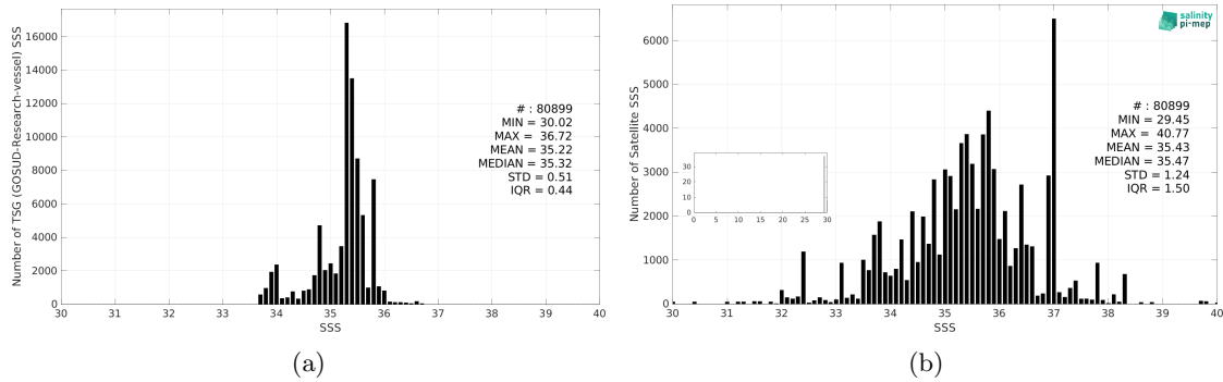
Figure 3: Histograms of SSS from TSG (GOSUD-Research-vessel) (a) and SMOS SSS L2Q v333 - 0.25 Deg (CATDS-CPDC) (b) considering all match-up pairs per bins of 0.1 over the Indian Ocean Pi-MEP region and for the full satellite product period.
