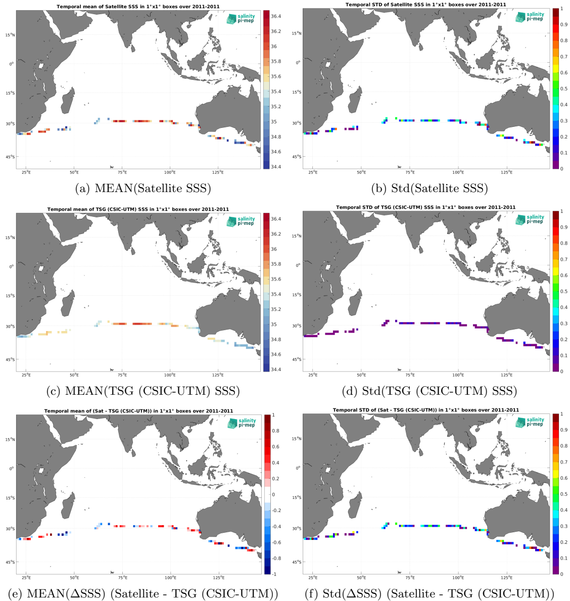
Figure 7: Temporal mean (left) and Std (right) of SSS from SMOS SSS L2Q v333 - 0.25 Deg (CATDS-CPDC) (top), TSG (CSIC-UTM) (middle), and of \Delta SSS (Satellite - TSG (CSIC-UTM)). Only match-up pairs are used to generate these maps.
