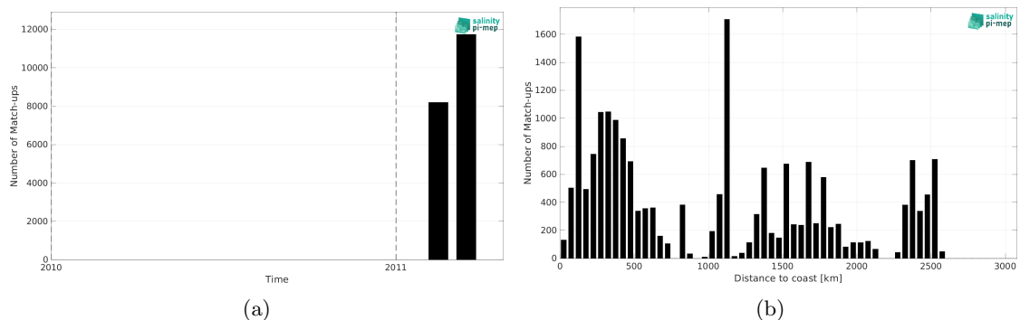
Figure 2: Number of match-ups between TSG (CSIC-UTM) and SMOS SSS L2Q v333 - 0.25 Deg (CATDS-CPDC) SSS as a function of time (a) and as function of the distance to coast (b) over the Indian Ocean Pi-MEP region and for the full satellite product period.
