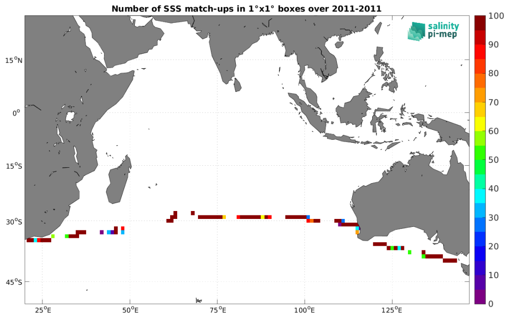
Figure 5: Number of SSS match-ups between TSG (CSIC-UTM) SSS and the SMOS SSS L2Q v333 - 0.25 Deg (CATDS-CPDC) SSS product for the Indian Ocean Pi-MEP region over 1^\circ \times 1^\circ boxes and for the full satellite product period.
