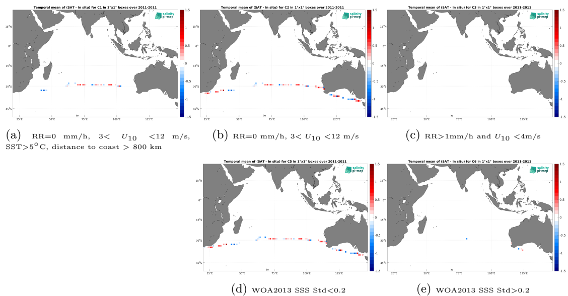
Figure 14: Temporal mean gridded over spatial boxes of size 1^\circ \times 1^\circ of \Delta SSS (SMOS SSS L2Q v333 - 0.25 Deg (CATDS-CPDC) - TSG (CSIC-UTM)) for 5 different subdatasets corresponding to: RR=0 mm/h, 3 < U_{10} < 12 m/s, SST > 5^\circ\text{C} , distance to coast > 800 km (a), RR=0 mm/h, 3 < U_{10} < 12 m/s (b), RR > 1 mm/h and U_{10} < 4 m/s (c), WOA2013 SSS Std < 0.2 (d), WOA2013 SSS Std > 0.2 (e).
