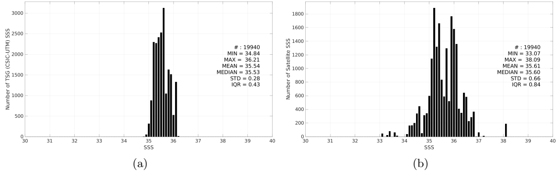
Figure 3: Histograms of SSS from TSG (CSIC-UTM) (a) and SMOS SSS L2Q v333 - 0.25 Deg (CATDS-CPDC) (b) considering all match-up pairs per bins of 0.1 over the Indian Ocean Pi-MEP region and for the full satellite product period.
