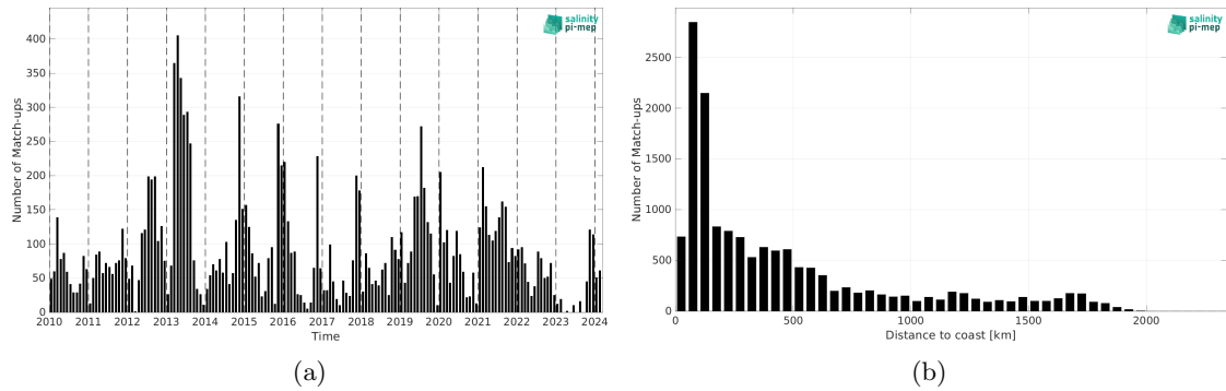
Figure 2: Number of match-ups between Marine mammals and SMOS SSS L2Q v333 - 0.25 Deg (CATDS-CPDC) SSS as a function of time (a) and as function of the distance to coast (b) over the Indian Ocean Pi-MEP region and for the full satellite product period.
