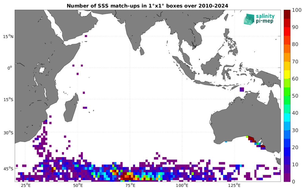
Figure 5: Number of SSS match-ups between Marine mammals SSS and the SMOS SSS L2Q v333 - 0.25 Deg (CATDS-CPDC) SSS product for the Indian Ocean Pi-MEP region over 1^\circ \times 1^\circ boxes and for the full satellite product period.
