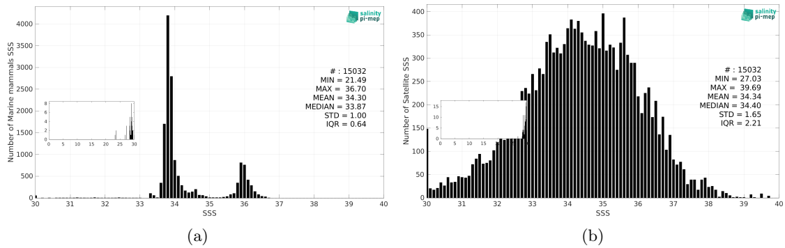
Figure 3: Histograms of SSS from Marine mammals (a) and SMOS SSS L2Q v333 - 0.25 Deg (CATDS-CPDC) (b) considering all match-up pairs per bins of 0.1 over the Indian Ocean Pi-MEP region and for the full satellite product period.
