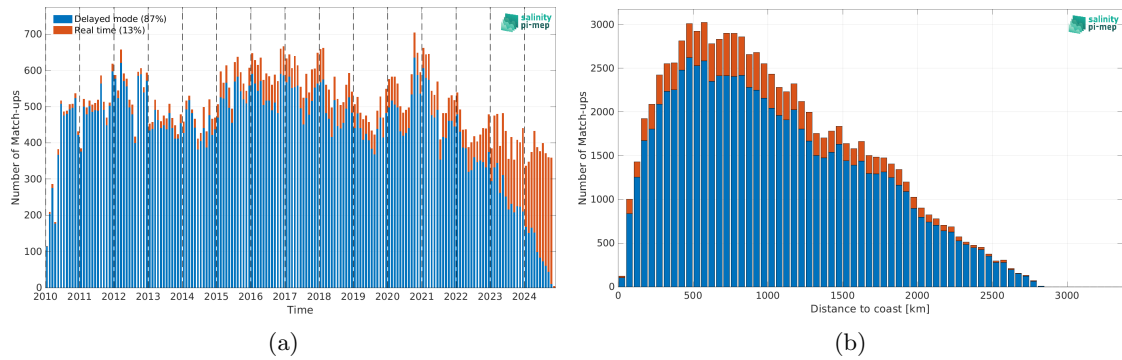
Figure 2: Number of match-ups between Argo and SMOS SSS L2Q v333 - 0.25 Deg (CATDS-CPDC) SSS as a function of time (a) and as function of the distance to coast (b) over the Indian Ocean Pi-MEP region and for the full satellite product period.
