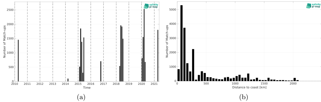
Figure 2: Number of match-ups between TSG (SAMOS) and SMOS SSS L3 v332 - 9 Days (CATDS-CPDC) SSS as a function of time (a) and as function of the distance to coast (b) over the Indian Ocean Pi-MEP region and for the full satellite product period.
