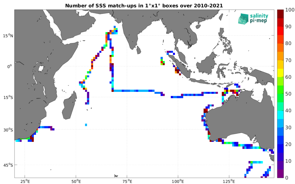
Figure 5: Number of SSS match-ups between TSG (SAMOS) SSS and the SMOS SSS L3 v332 - 9 Days (CATDS-CPDC) SSS product for the Indian Ocean Pi-MEP region over 1^\circ \times 1^\circ boxes and for the full satellite product period.
