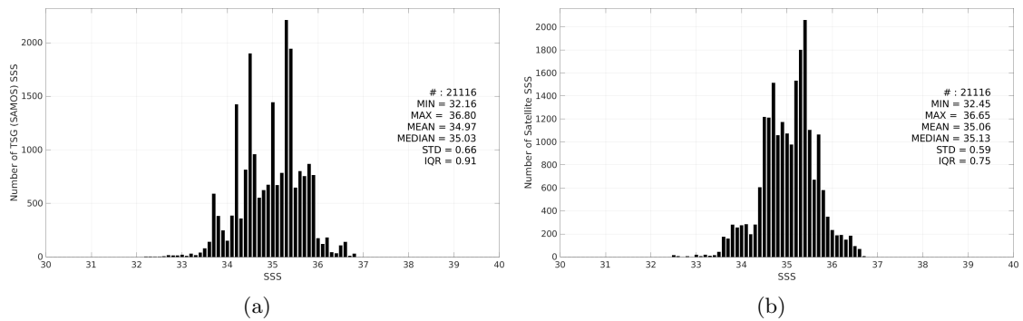
Figure 3: Histograms of SSS from TSG (SAMOS) (a) and SMOS SSS L3 v332 - 9 Days (CATDS-CPDC) (b) considering all match-up pairs per bins of 0.1 over the Indian Ocean Pi-MEP region and for the full satellite product period.
