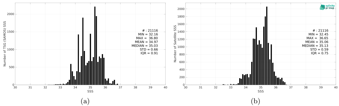
Figure 2: Histograms of SSS from TSG (SAMOS) (a) and SMOS SSS L3 v332 - 9 Days (CATDS-CPDC) (b) considering all match-up pairs per bins of 0.1 over the Indian Ocean Pi-MEP region and for the full satellite product period.
