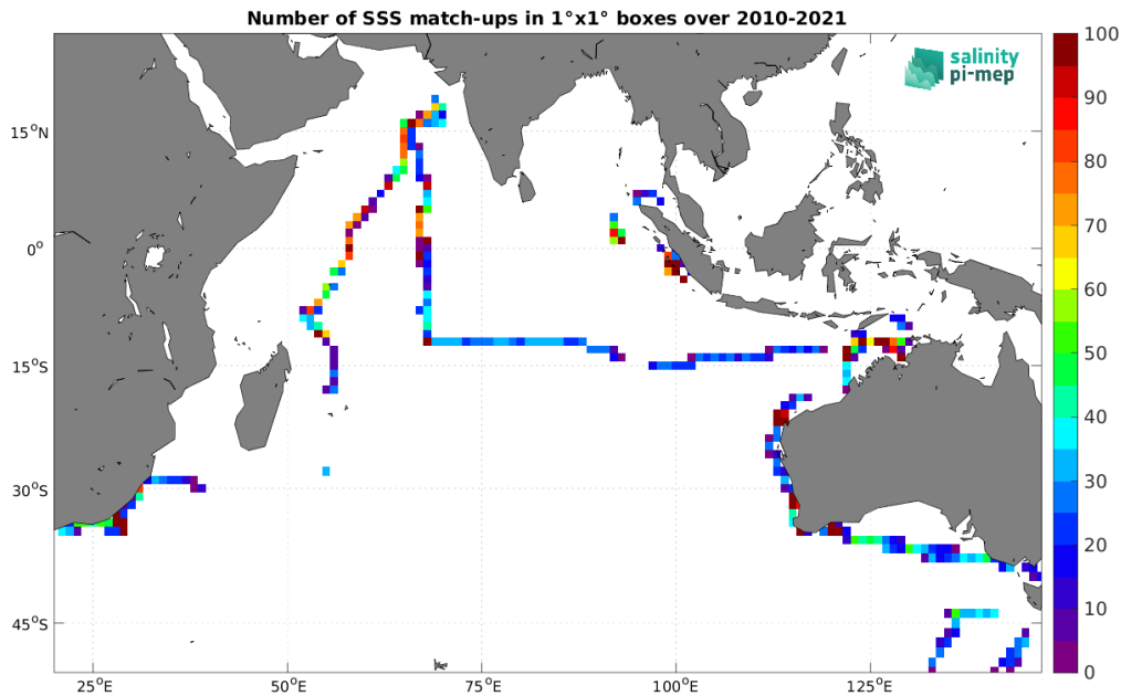
Figure 4: Number of SSS match-ups between TSG (SAMOS) SSS and the SMOS SSS L3 v332 - 9 Days (CATDS-CPDC) SSS product for the Indian Ocean Pi-MEP region over 1^\circ \times 1^\circ boxes and for the full satellite product period.
