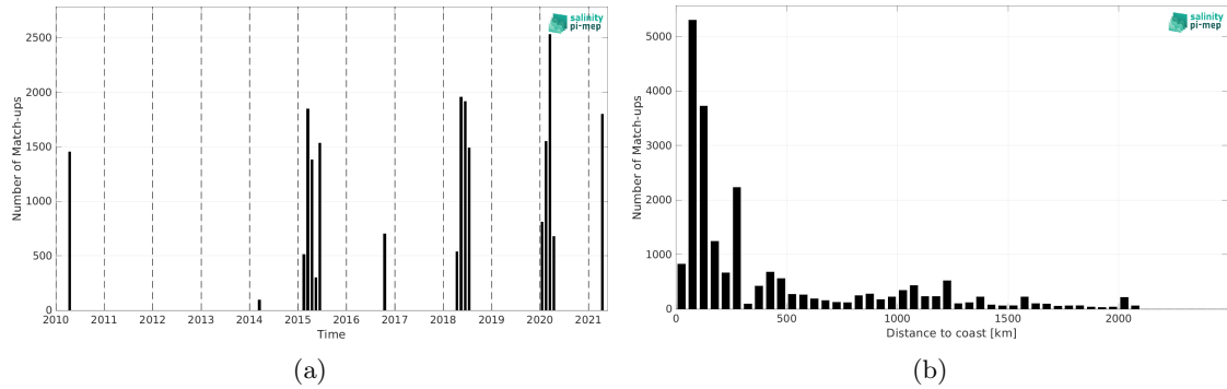
Figure 1: Number of match-ups between TSG (SAMOS) and SMOS SSS L3 v332 - 9 Days (CATDS-CPDC) SSS as a function of time (a) and as function of the distance to coast (b) over the Indian Ocean Pi-MEP region and for the full satellite product period.
