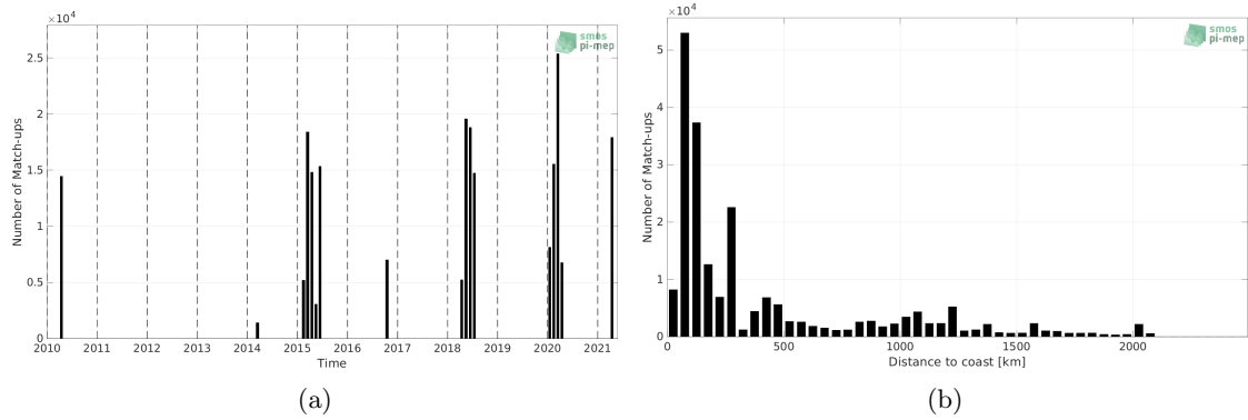
Figure 1: Number of match-ups between TSG (SAMOS) and SMOS SSS L3 v332 - 9 Days (CATDS-CPDC) SSS as a function of time (a) and as function of the distance to coast (b) over the Indian Ocean Pi-MEP region and for the full satellite product period.
