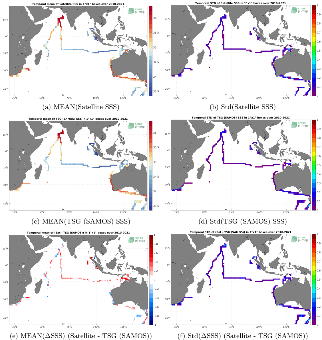
Figure 6: Temporal mean (left) and Std (right) of SSS from SMOS SSS L3 v332 - 9 Days (CATDS-CPDC) (top), TSG (SAMOS) (middle), and of \Delta SSS (Satellite - TSG (SAMOS)). Only match-up pairs are used to generate these maps.
