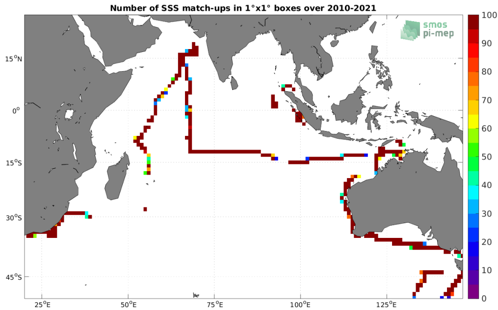
Figure 4: Number of SSS match-ups between TSG (SAMOS) SSS and the SMOS SSS L3 v332 - 9 Days (CATDS-CPDC) SSS product for the Indian Ocean Pi-MEP region over 1^\circ \times 1^\circ boxes and for the full satellite product period.
