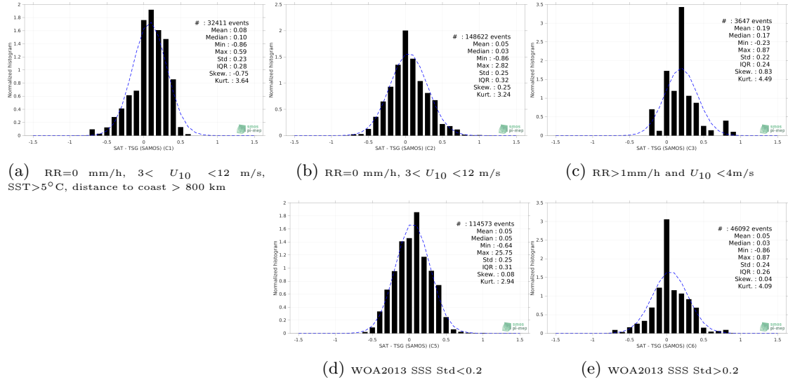
Figure 13: Normalized histogram of \Delta SSS (SMOS SSS L3 v332 - 9 Days (CATDS-CPDC) - TSG (SAMOS)) for 5 different subdatasets corresponding to: RR=0 mm/h, 3 < U_{10} < 12 m/s, SST > 5°C, distance to coast > 800 km (a), RR=0 mm/h, 3 < U_{10} < 12 m/s (b), RR > 1mm/h and U_{10} < 4 m/s (c), WOA2013 SSS Std < 0.2 (d), WOA2013 SSS Std > 0.2 (e).
