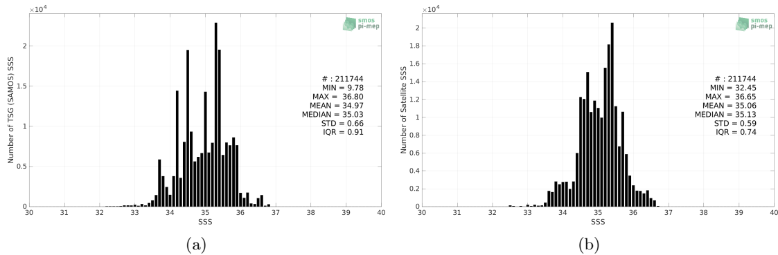
Figure 2: Histograms of SSS from TSG (SAMOS) (a) and SMOS SSS L3 v332 - 9 Days (CATDS-CPDC) (b) considering all match-up pairs per bins of 0.1 over the Indian Ocean Pi-MEP region and for the full satellite product period.
