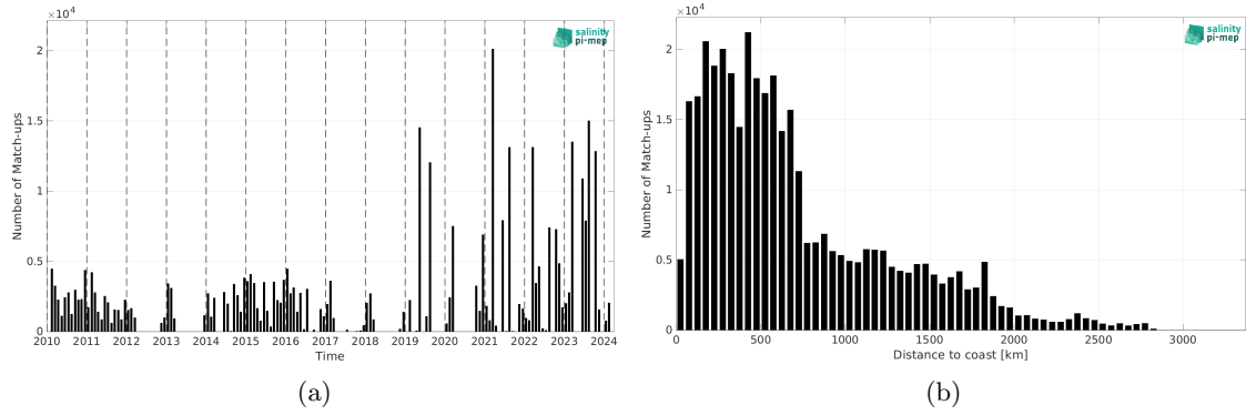
Figure 2: Number of match-ups between TSG (LEGOS-DM) and SMOS SSS L3 v332 - 9 Days (CATDS-CPDC) SSS as a function of time (a) and as function of the distance to coast (b) over the Indian Ocean Pi-MEP region and for the full satellite product period.
