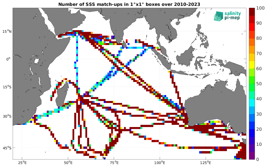
Figure 5: Number of SSS match-ups between TSG (LEGOS-DM) SSS and the SMOS SSS L3 v332 - 9 Days (CATDS-CPDC) SSS product for the Indian Ocean Pi-MEP region over 1^\circ \times 1^\circ boxes and for the full satellite product period.
