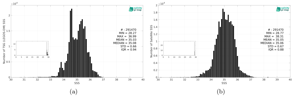
Figure 3: Histograms of SSS from TSG (LEGOS-DM) (a) and SMOS SSS L3 v332 - 9 Days (CATDS-CPDC) (b) considering all match-up pairs per bins of 0.1 over the Indian Ocean Pi-MEP region and for the full satellite product period.
