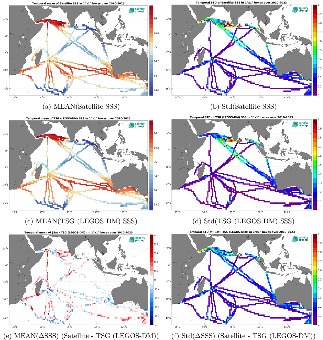
Figure 7: Temporal mean (left) and Std (right) of SSS from SMOS SSS L3 v332 - 9 Days (CATDS-CPDC) (top), TSG (LEGOS-DM) (middle), and of \Delta SSS (Satellite - TSG (LEGOS-DM)). Only match-up pairs are used to generate these maps.
