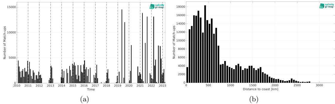
Figure 2: Number of match-ups between TSG (LEGOS-DM) and SMOS SSS L3 v332 - 9 Days (CATDS-CPDC) SSS as a function of time (a) and as function of the distance to coast (b) over the Indian Ocean Pi-MEP region and for the full satellite product period.
