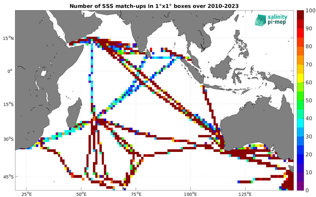
Figure 4: Number of SSS match-ups between TSG (LEGOS-DM) SSS and the SMOS SSS L3 v332 - 9 Days (CATDS-CPDC) SSS product for the Indian Ocean Pi-MEP region over 1^\circ \times 1^\circ boxes and for the full satellite product period.
