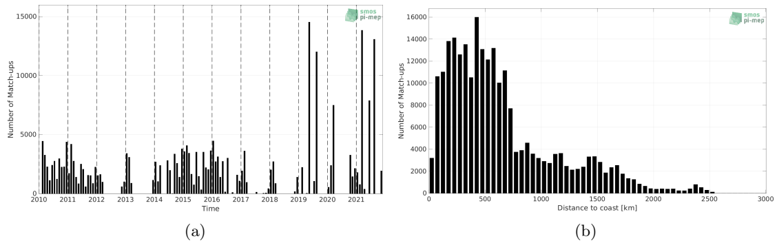
Figure 1: Number of match-ups between TSG (LEGOS-DM) and SMOS SSS L3 v332 - 9 Days (CATDS-CPDC) SSS as a function of time (a) and as function of the distance to coast (b) over the Indian Ocean Pi-MEP region and for the full satellite product period.
