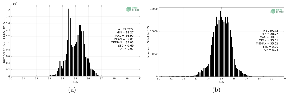
Figure 2: Histograms of SSS from TSG (LEGOS-DM) (a) and SMOS SSS L3 v332 - 9 Days (CATDS-CPDC) (b) considering all match-up pairs per bins of 0.1 over the Indian Ocean Pi-MEP region and for the full satellite product period.
