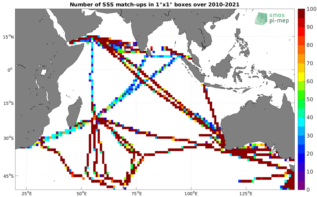
Figure 4: Number of SSS match-ups between TSG (LEGOS-DM) SSS and the SMOS SSS L3 v332 - 9 Days (CATDS-CPDC) SSS product for the Indian Ocean Pi-MEP region over 1^\circ \times 1^\circ boxes and for the full satellite product period.
