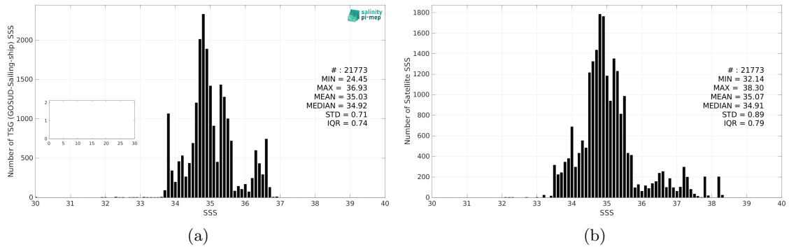
Figure 3: Histograms of SSS from TSG (GOSUD-Sailing-ship) (a) and SMOS SSS L3 v332 - 9 Days (CATDS-CPDC) (b) considering all match-up pairs per bins of 0.1 over the Indian Ocean Pi-MEP region and for the full satellite product period.
