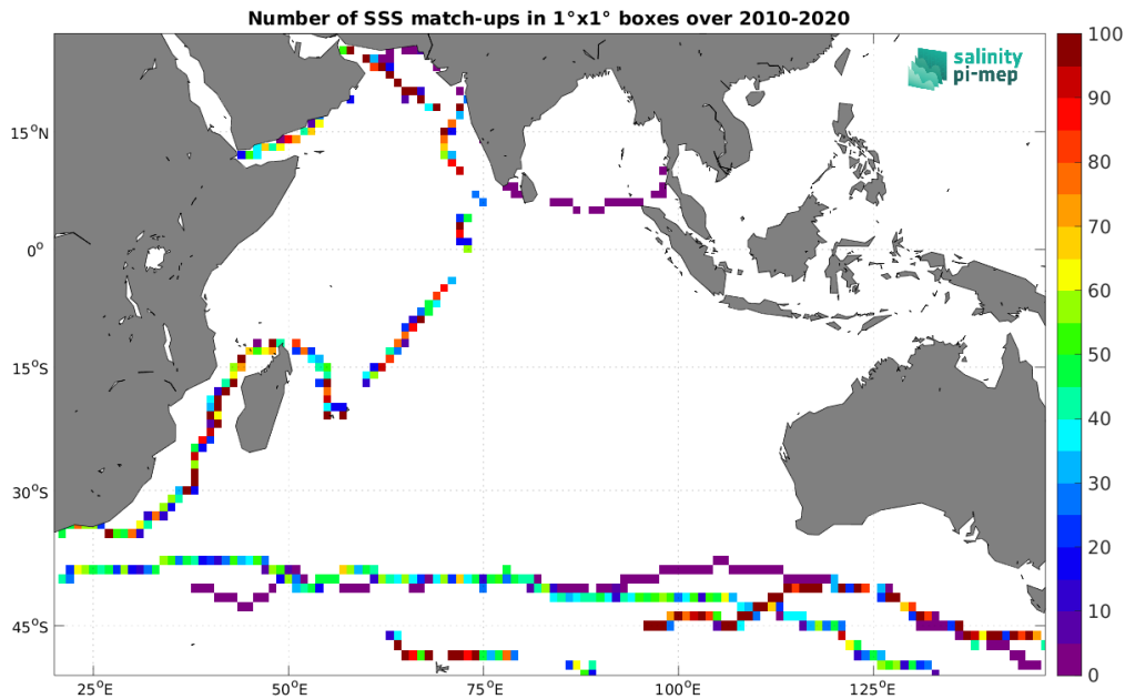
Figure 5: Number of SSS match-ups between TSG (GOSUD-Sailing-ship) SSS and the SMOS SSS L3 v332 - 9 Days (CATDS-CPDC) SSS product for the Indian Ocean Pi-MEP region over 1^\circ \times 1^\circ boxes and for the full satellite product period.
