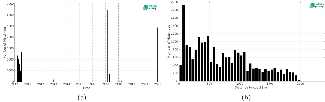
Figure 2: Number of match-ups between TSG (GOSUD-Sailing-ship) and SMOS SSS L3 v332 - 9 Days (CATDS-CPDC) SSS as a function of time (a) and as function of the distance to coast (b) over the Indian Ocean Pi-MEP region and for the full satellite product period.
