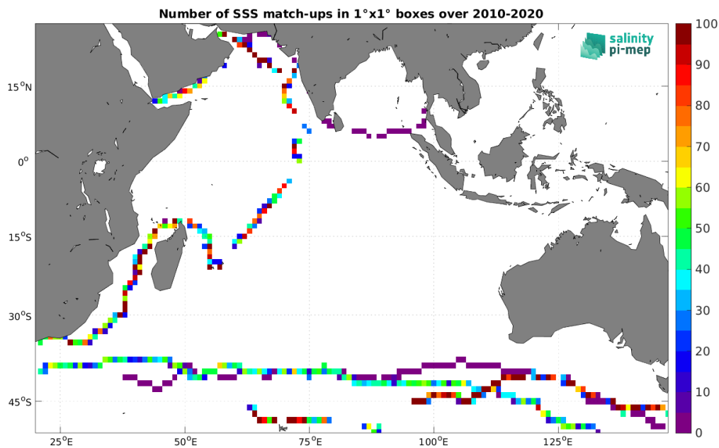
Figure 4: Number of SSS match-ups between TSG (GOSUD-Sailing-ship) SSS and the SMOS SSS L3 v332 - 9 Days (CATDS-CPDC) SSS product for the Indian Ocean Pi-MEP region over 1^\circ \times 1^\circ boxes and for the full satellite product period.
