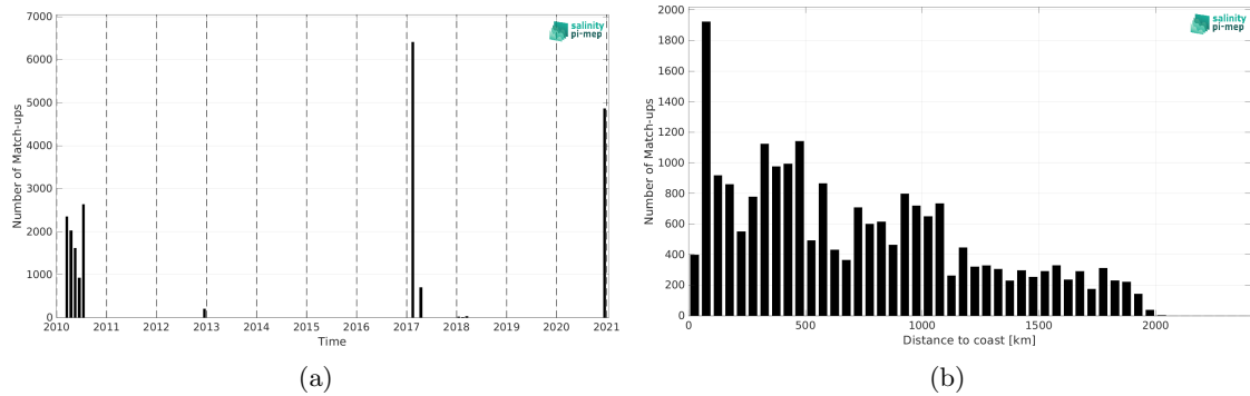
Figure 1: Number of match-ups between TSG (GOSUD-Sailing-ship) and SMOS SSS L3 v332 - 9 Days (CATDS-CPDC) SSS as a function of time (a) and as function of the distance to coast (b) over the Indian Ocean Pi-MEP region and for the full satellite product period.
