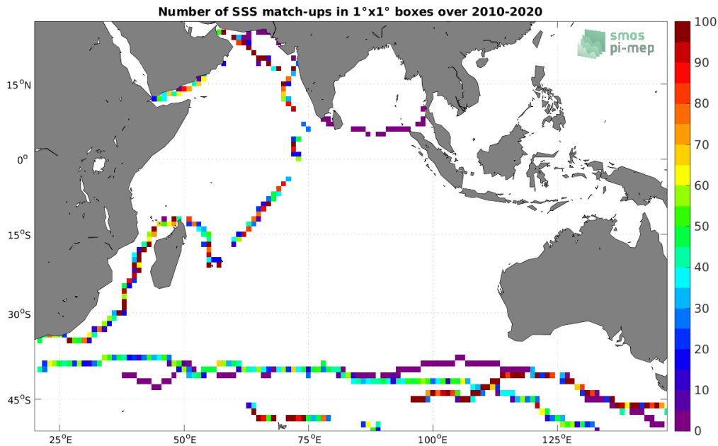
Figure 4: Number of SSS match-ups between TSG (GOSUD-Sailing-ship) SSS and the SMOS SSS L3 v332 - 9 Days (CATDS-CPDC) SSS product for the Indian Ocean Pi-MEP region over 1^\circ \times 1^\circ boxes and for the full satellite product period.
