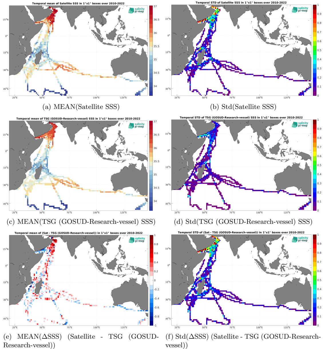
Figure 7: Temporal mean (left) and Std (right) of SSS from SMOS SSS L3 v332 - 9 Days (CATDS-CPDC) (top), TSG (GOSUD-Research-vessel) (middle), and of \Delta SSS (Satellite - TSG (GOSUD-Research-vessel)). Only match-up pairs are used to generate these maps.
