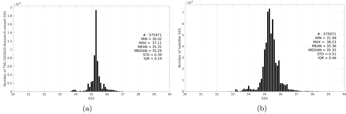
Figure 3: Histograms of SSS from TSG (GOSUD-Research-vessel) (a) and SMOS SSS L3 v332 - 9 Days (CATDS-CPDC) (b) considering all match-up pairs per bins of 0.1 over the Indian Ocean Pi-MEP region and for the full satellite product period.
