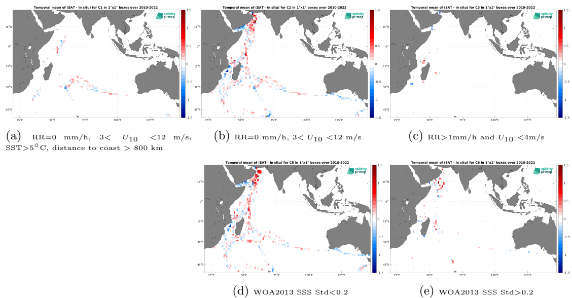
Figure 14: Temporal mean gridded over spatial boxes of size 1^\circ \times 1^\circ of \Delta SSS (SMOS SSS L3 v332 - 9 Days (CATDS-CPDC) - TSG (GOSUD-Research-vessel)) for 5 different subdatasets corresponding to:RR=0 mm/h, 3 < U_{10} < 12 m/s, SST >5^\circ\text{C} , distance to coast > 800 km (a), RR=0 mm/h, 3 < U_{10} < 12 m/s (b), RR >1 mm/h and U_{10} < 4 m/s (c), WOA2013 SSS Std <0.2 (d), WOA2013 SSS Std >0.2 (e).
