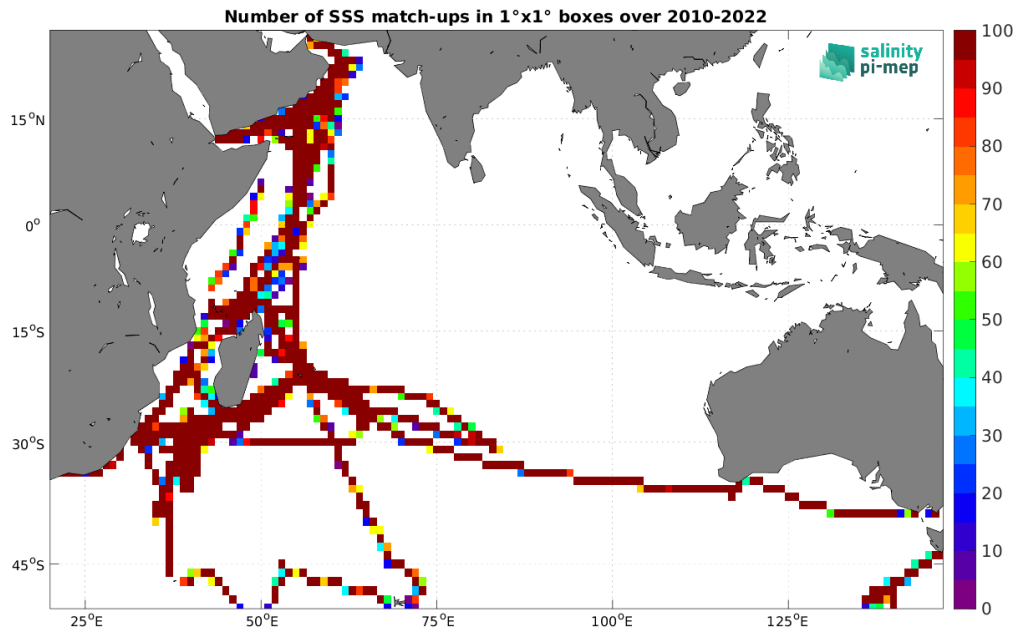
Figure 5: Number of SSS match-ups between TSG (GOSUD-Research-vessel) SSS and the SMOS SSS L3 v332 - 9 Days (CATDS-CPDC) SSS product for the Indian Ocean Pi-MEP region over 1^\circ \times 1^\circ boxes and for the full satellite product period.
