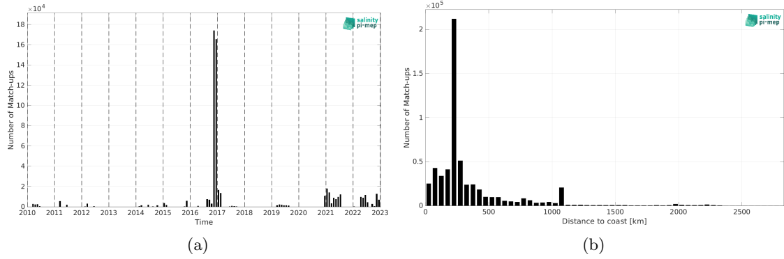
Figure 2: Number of match-ups between TSG (GOSUD-Research-vessel) and SMOS SSS L3 v332 - 9 Days (CATDS-CPDC) SSS as a function of time (a) and as function of the distance to coast (b) over the Indian Ocean Pi-MEP region and for the full satellite product period.
