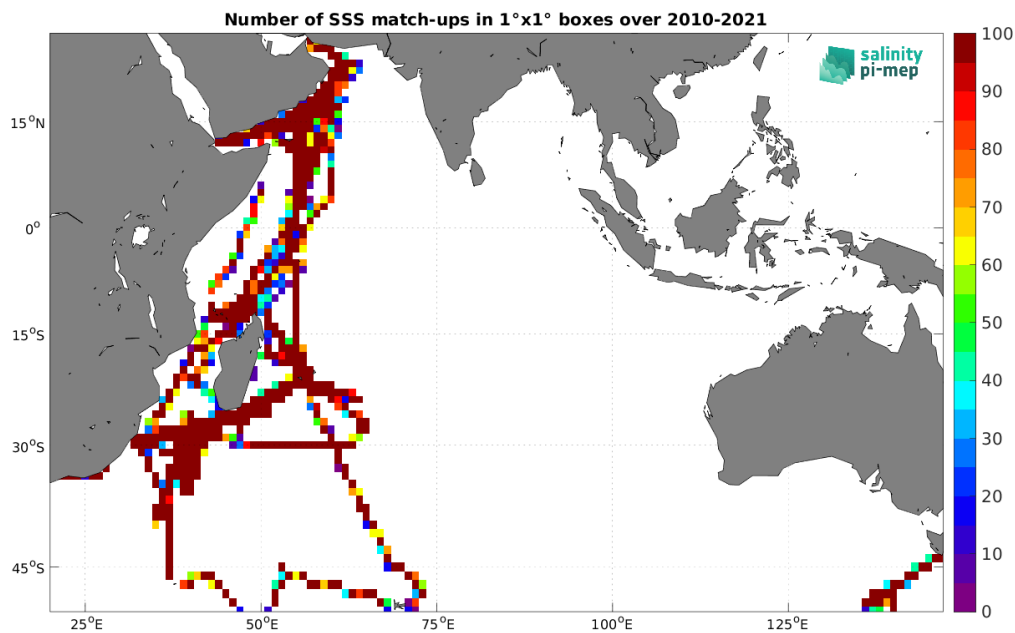
Figure 4: Number of SSS match-ups between TSG (GOSUD-Research-vessel) SSS and the SMOS SSS L3 v332 - 9 Days (CATDS-CPDC) SSS product for the Indian Ocean Pi-MEP region over 1^\circ \times 1^\circ boxes and for the full satellite product period.
