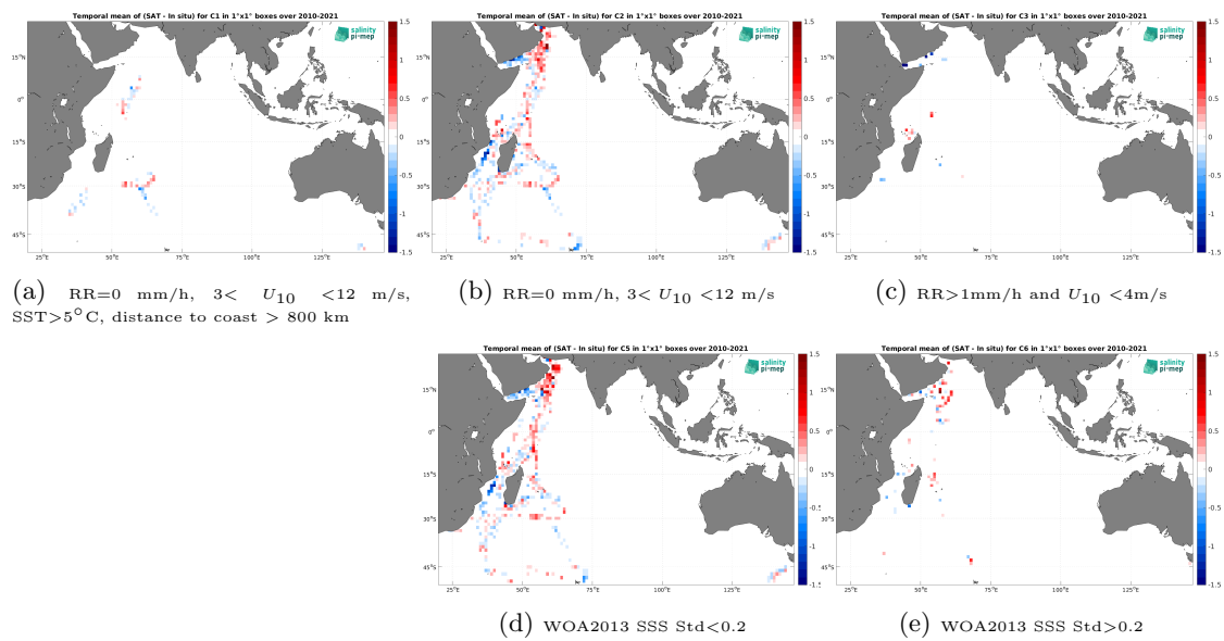
Figure 12: Temporal mean gridded over spatial boxes of size 1^\circ \times 1^\circ of \Delta SSS (SMOS SSS L3 v332 - 9 Days (CATDS-CPDC) - TSG (GOSUD-Research-vessel)) for 5 different subdatasets corresponding to:RR=0 mm/h, 3 < U_{10} < 12 m/s, SST >5^\circ\text{C} , distance to coast > 800 km (a), RR=0 mm/h, 3 < U_{10} < 12 m/s (b), RR >1 mm/h and U_{10} < 4 m/s (c), WOA2013 SSS Std <0.2 (d), WOA2013 SSS Std >0.2 (e).
