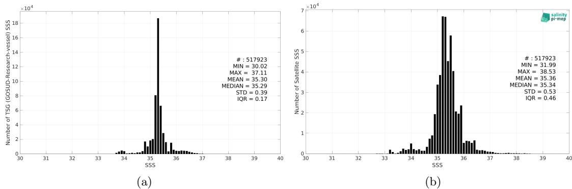
Figure 2: Histograms of SSS from TSG (GOSUD-Research-vessel) (a) and SMOS SSS L3 v332 - 9 Days (CATDS-CPDC) (b) considering all match-up pairs per bins of 0.1 over the Indian Ocean Pi-MEP region and for the full satellite product period.
