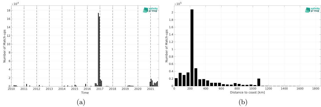
Figure 1: Number of match-ups between TSG (GOSUD-Research-vessel) and SMOS SSS L3 v332 - 9 Days (CATDS-CPDC) SSS as a function of time (a) and as function of the distance to coast (b) over the Indian Ocean Pi-MEP region and for the full satellite product period.
