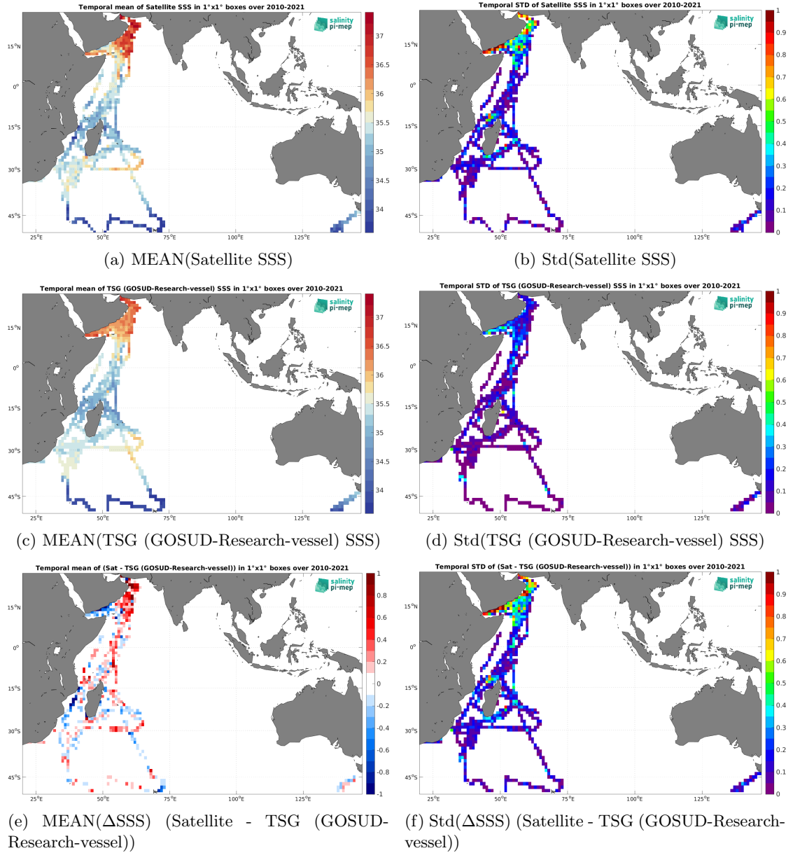
Figure 6: Temporal mean (left) and Std (right) of SSS from SMOS SSS L3 v332 - 9 Days (CATDS-CPDC) (top), TSG (GOSUD-Research-vessel) (middle), and of \Delta SSS (Satellite - TSG (GOSUD-Research-vessel)). Only match-up pairs are used to generate these maps.
