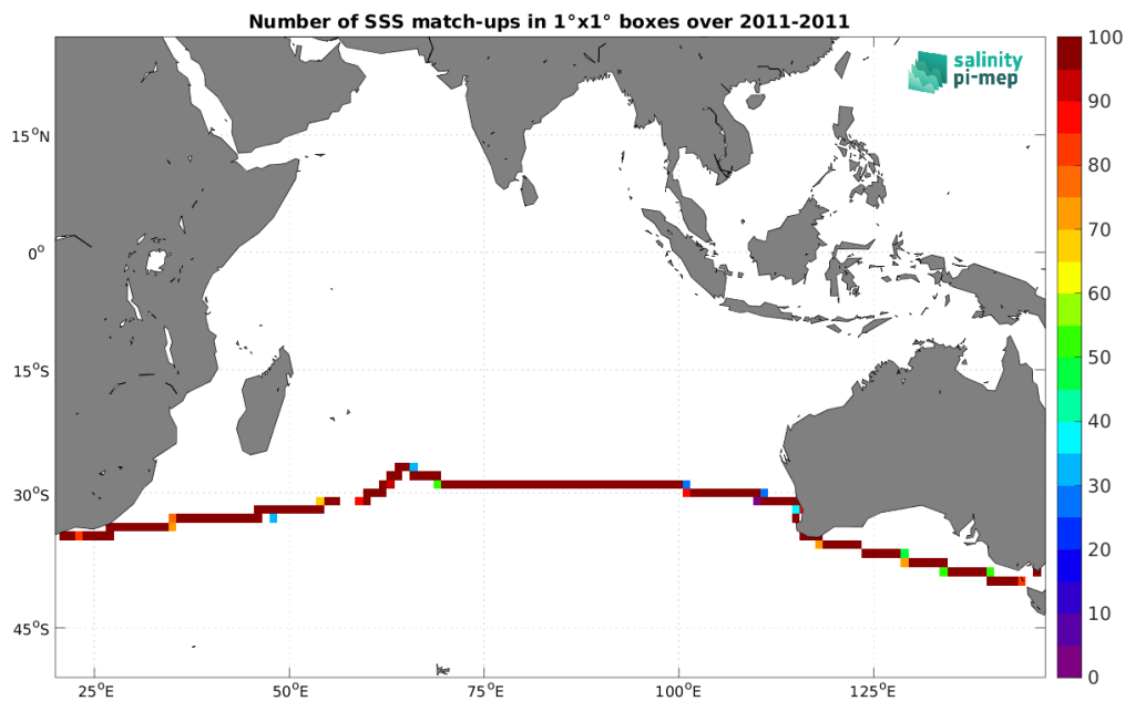
Figure 5: Number of SSS match-ups between TSG (CSIC-UTM) SSS and the SMOS SSS L3 v332 - 9 Days (CATDS-CPDC) SSS product for the Indian Ocean Pi-MEP region over 1^\circ \times 1^\circ boxes and for the full satellite product period.
