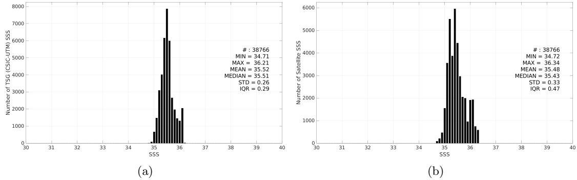
Figure 3: Histograms of SSS from TSG (CSIC-UTM) (a) and SMOS SSS L3 v332 - 9 Days (CATDS-CPDC) (b) considering all match-up pairs per bins of 0.1 over the Indian Ocean Pi-MEP region and for the full satellite product period.
