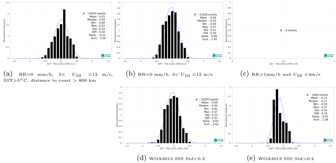
Figure 15: Normalized histogram of \Delta SSS (SMOS SSS L3 v332 - 9 Days (CATDS-CPDC) - TSG (CSIC-UTM)) for 5 different subdatasets corresponding to: RR=0 mm/h, 3 < U_{10} < 12 m/s, SST > 5°C, distance to coast > 800 km (a), RR=0 mm/h, 3 < U_{10} < 12 m/s (b), RR > 1mm/h and U_{10} < 4 m/s (c), WOA2013 SSS Std < 0.2 (d), WOA2013 SSS Std > 0.2 (e).
