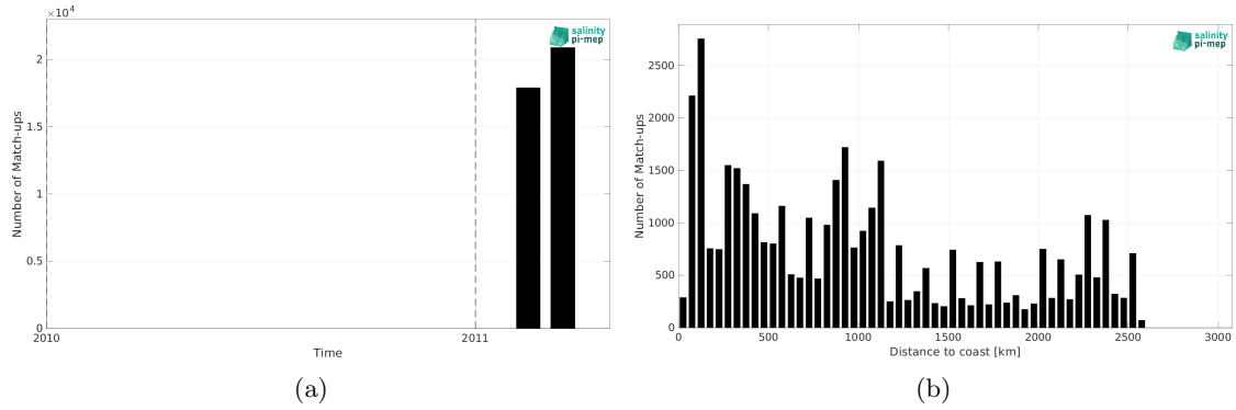
Figure 2: Number of match-ups between TSG (CSIC-UTM) and SMOS SSS L3 v332 - 9 Days (CATDS-CPDC) SSS as a function of time (a) and as function of the distance to coast (b) over the Indian Ocean Pi-MEP region and for the full satellite product period.
