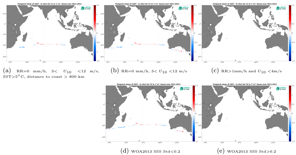
Figure 14: Temporal mean gridded over spatial boxes of size 1^\circ \times 1^\circ of \Delta SSS (SMOS SSS L3 v332 - 9 Days (CATDS-CPDC) - TSG (CSIC-UTM)) for 5 different subdatasets corresponding to: RR=0 mm/h, 3 < U_{10} < 12 m/s, SST > 5^\circ\text{C} , distance to coast > 800 km (a), RR=0 mm/h, 3 < U_{10} < 12 m/s (b), RR > 1\text{mm/h} and U_{10} < 4\text{m/s} (c), WOA2013 SSS Std < 0.2 (d), WOA2013 SSS Std > 0.2 (e).
