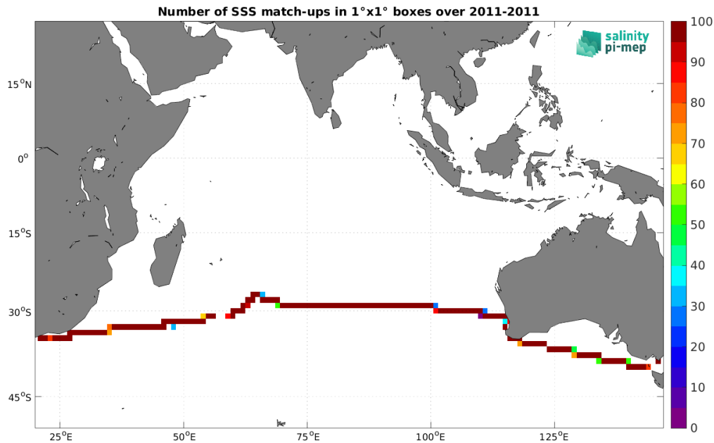
Figure 5: Number of SSS match-ups between TSG (CSIC-UTM) SSS and the SMOS SSS L3 v332 - 9 Days (CATDS-CPDC) SSS product for the Indian Ocean Pi-MEP region over 1^\circ \times 1^\circ boxes and for the full satellite product period.
