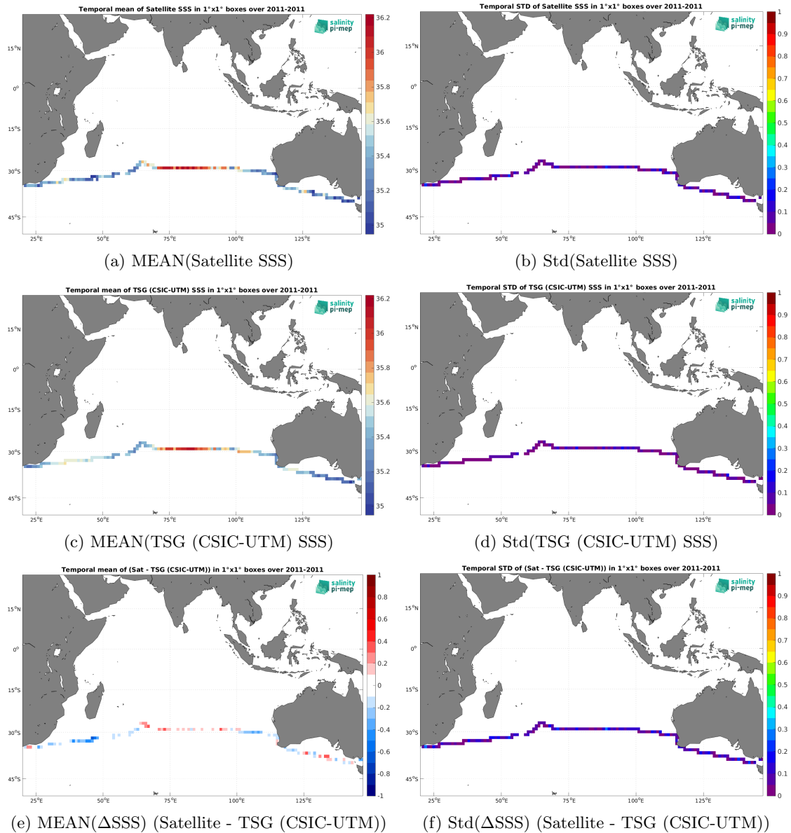
Figure 7: Temporal mean (left) and Std (right) of SSS from SMOS SSS L3 v332 - 9 Days (CATDS-CPDC) (top), TSG (CSIC-UTM) (middle), and of \Delta SSS (Satellite - TSG (CSIC-UTM)). Only match-up pairs are used to generate these maps.
