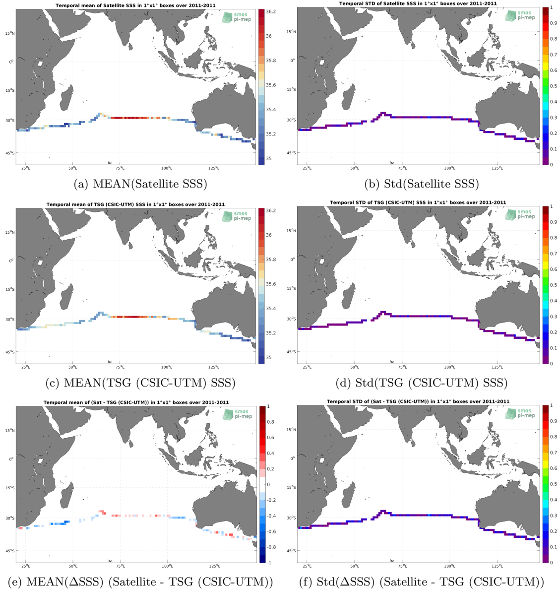
Figure 6: Temporal mean (left) and Std (right) of SSS from SMOS SSS L3 v332 - 9 Days (CATDS-CPDC) (top), TSG (CSIC-UTM) (middle), and of \Delta SSS (Satellite - TSG (CSIC-UTM)). Only match-up pairs are used to generate these maps.
