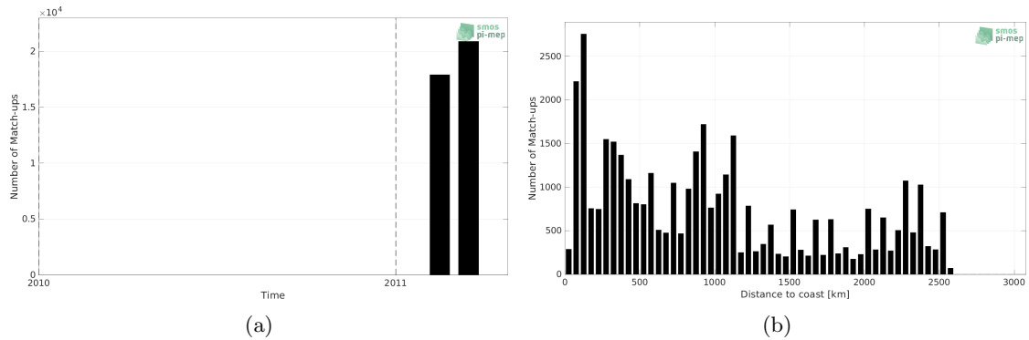
Figure 1: Number of match-ups between TSG (CSIC-UTM) and SMOS SSS L3 v332 - 9 Days (CATDS-CPDC) SSS as a function of time (a) and as function of the distance to coast (b) over the Indian Ocean Pi-MEP region and for the full satellite product period.
