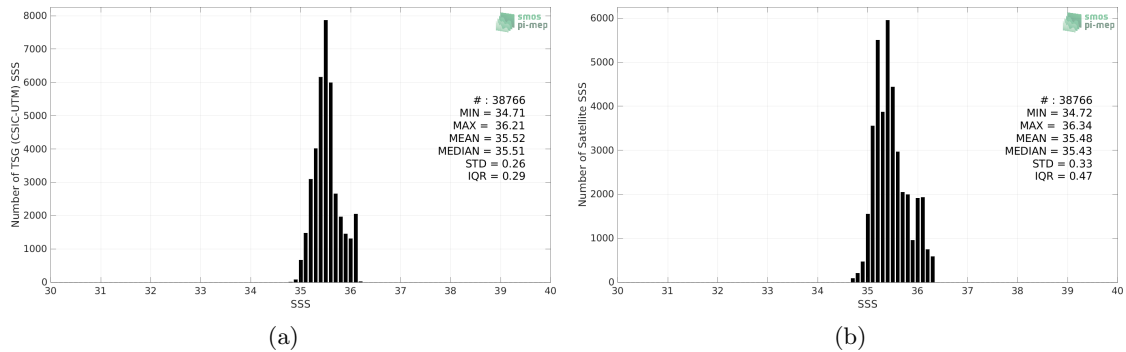
Figure 2: Histograms of SSS from TSG (CSIC-UTM) (a) and SMOS SSS L3 v332 - 9 Days (CATDS-CPDC) (b) considering all match-up pairs per bins of 0.1 over the Indian Ocean Pi-MEP region and for the full satellite product period.
