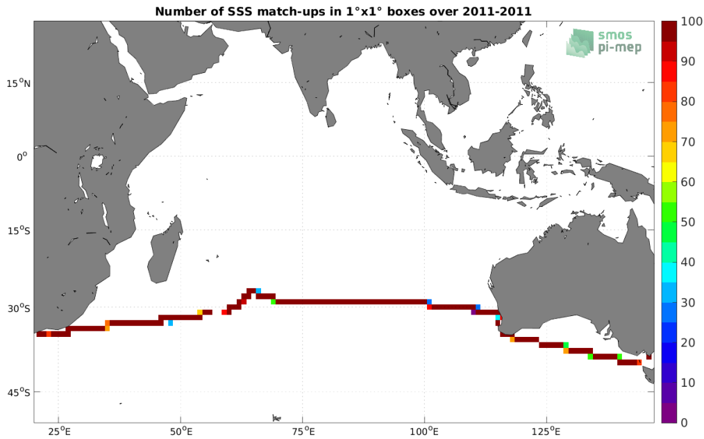
Figure 4: Number of SSS match-ups between TSG (CSIC-UTM) SSS and the SMOS SSS L3 v332 - 9 Days (CATDS-CPDC) SSS product for the Indian Ocean Pi-MEP region over 1^\circ \times 1^\circ boxes and for the full satellite product period.
