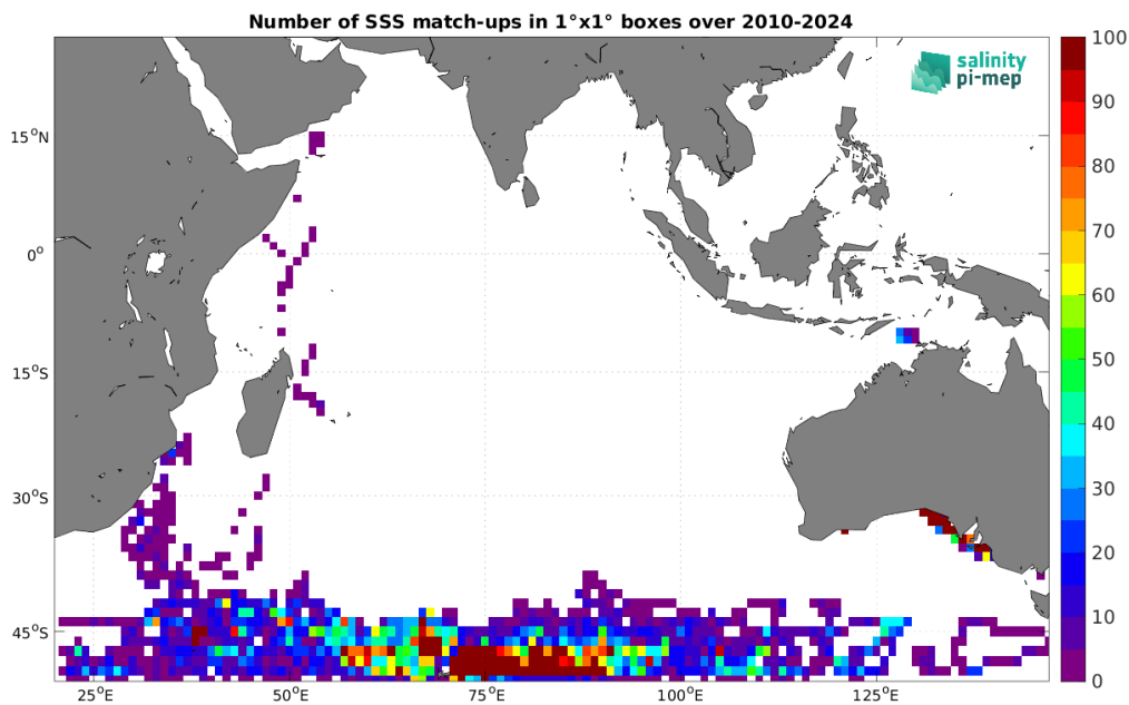
Figure 5: Number of SSS match-ups between Marine mammals SSS and the SMOS SSS L3 v332 - 9 Days (CATDS-CPDC) SSS product for the Indian Ocean Pi-MEP region over 1^\circ \times 1^\circ boxes and for the full satellite product period.
