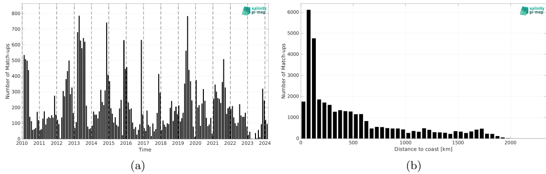
Figure 2: Number of match-ups between Marine mammals and SMOS SSS L3 v332 - 9 Days (CATDS-CPDC) SSS as a function of time (a) and as function of the distance to coast (b) over the Indian Ocean Pi-MEP region and for the full satellite product period.
