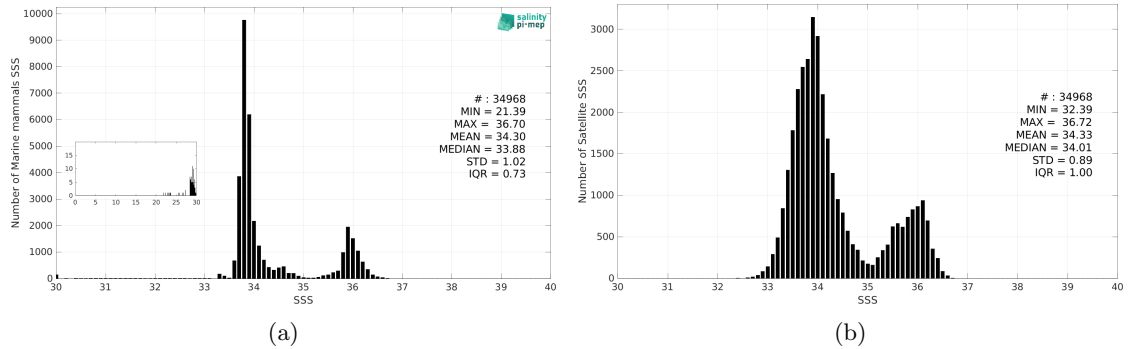
Figure 3: Histograms of SSS from Marine mammals (a) and SMOS SSS L3 v332 - 9 Days (CATDS-CPDC) (b) considering all match-up pairs per bins of 0.1 over the Indian Ocean Pi-MEP region and for the full satellite product period.
