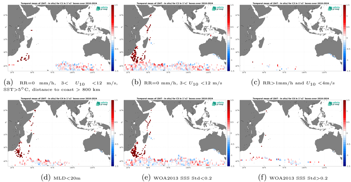
Figure 14: Temporal mean gridded over spatial boxes of size 1^\circ \times 1^\circ of \Delta\text{SSS} (SMOS SSS L3 v332 - 9 Days (CATDS-CPDC) - Marine mammals) for 6 different subdatasets corresponding to: RR=0 mm/h, 3 < U_{10} < 12 m/s, SST > 5°C, distance to coast > 800 km (a), RR=0 mm/h, 3 < U_{10} < 12 m/s (b), RR > 1mm/h and U_{10} < 4 m/s (c), MLD < 20m (d), WOA2013 SSS Std < 0.2 (e), WOA2013 SSS Std > 0.2 (f).
