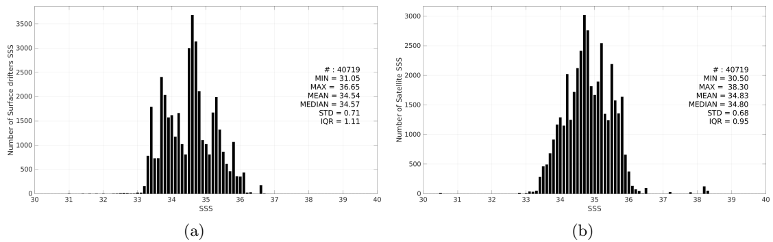
Figure 3: Histograms of SSS from Surface drifters (a) and SMOS SSS L3 v332 - 9 Days (CATDS-CPDC) (b) considering all match-up pairs per bins of 0.1 over the Indian Ocean Pi-MEP region and for the full satellite product period.
