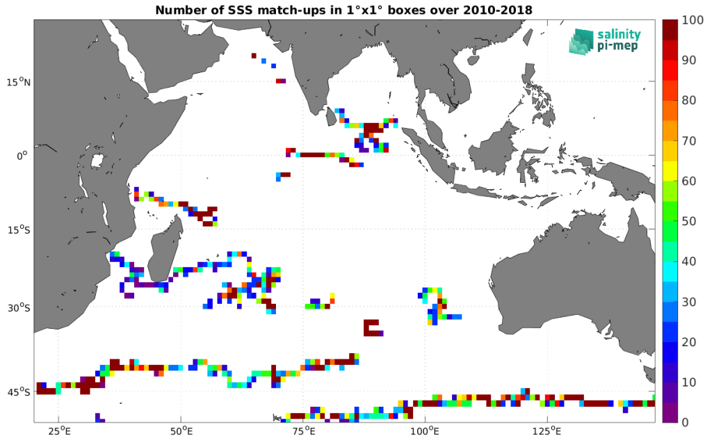
Figure 4: Number of SSS match-ups between Surface drifters SSS and the SMOS SSS L3 v332 - 9 Days (CATDS-CPDC) SSS product for the Indian Ocean Pi-MEP region over 1^\circ \times 1^\circ boxes and for the full satellite product period.
