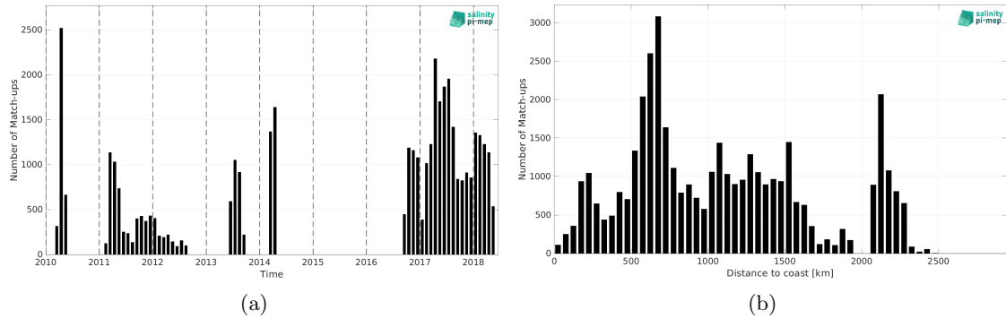
Figure 2: Number of match-ups between Surface drifters and SMOS SSS L3 v332 - 9 Days (CATDS-CPDC) SSS as a function of time (a) and as function of the distance to coast (b) over the Indian Ocean Pi-MEP region and for the full satellite product period.
