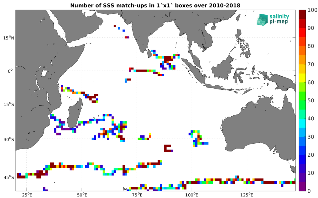
Figure 4: Number of SSS match-ups between Surface drifters SSS and the SMOS SSS L3 v332 - 9 Days (CATDS-CPDC) SSS product for the Indian Ocean Pi-MEP region over 1^\circ \times 1^\circ boxes and for the full satellite product period.
