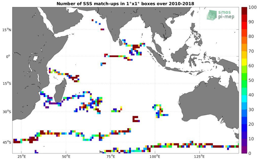
Figure 3: Number of SSS match-ups between Surface drifters SSS and the SMOS SSS L3 v332 - 9 Days (CATDS-CPDC) SSS product for the Indian Ocean Pi-MEP region over 1^\circ \times 1^\circ boxes and for the full satellite product period.
