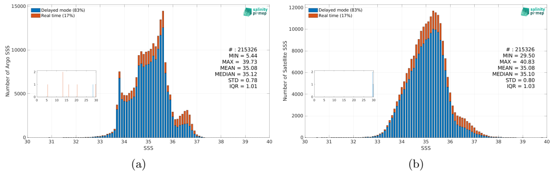
Figure 3: Histograms of SSS from Argo (a) and SMOS SSS L3 v332 - 9 Days (CATDS-CPDC) (b) considering all match-up pairs per bins of 0.1 over the Indian Ocean Pi-MEP region and for the full satellite product period.
