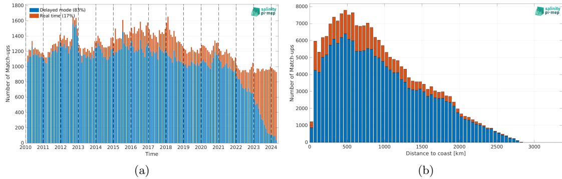
Figure 2: Number of match-ups between Argo and SMOS SSS L3 v332 - 9 Days (CATDS-CPDC) SSS as a function of time (a) and as function of the distance to coast (b) over the Indian Ocean Pi-MEP region and for the full satellite product period.
