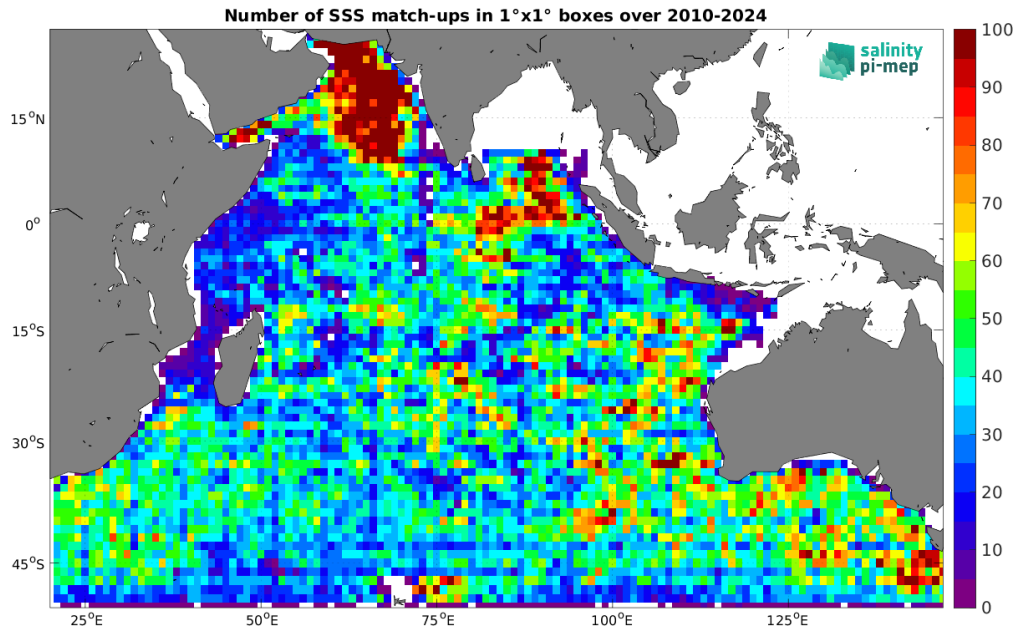
Figure 5: Number of SSS match-ups between Argo SSS and the SMOS SSS L3 v332 - 9 Days (CATDS-CPDC) SSS product for the Indian Ocean Pi-MEP region over 1^\circ \times 1^\circ boxes and for the full satellite product period.
