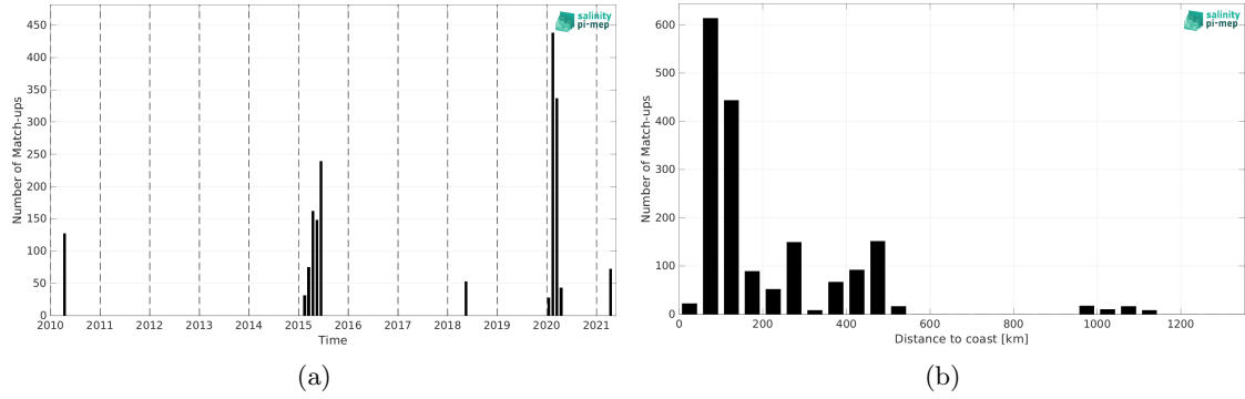
Figure 1: Number of match-ups between TSG (SAMOS) and SMOS SSS L2Q v331 - 0.25 Deg (CATDS-CPDC) SSS as a function of time (a) and as function of the distance to coast (b) over the Indian Ocean Pi-MEP region and for the full satellite product period.
