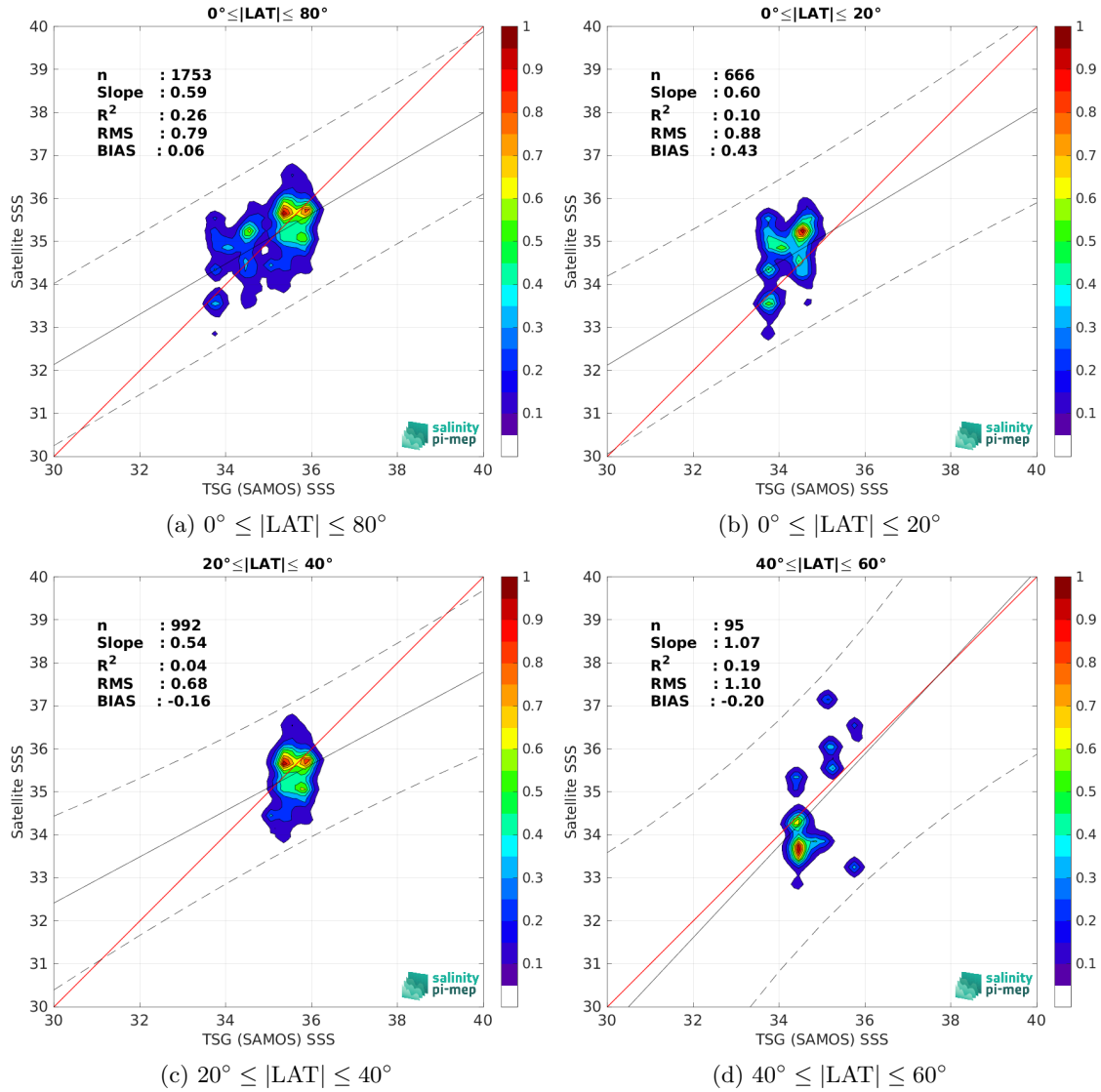
Figure 9: Contour maps of the concentration of SMOS SSS L2Q v331 - 0.25 Deg (CATDS-CPDC) SSS (y-axis) versus TSG (SAMOS) SSS (x-axis) at match-up pairs for different latitude bands. For each plot, the red line shows x=y . The black thin and dashed lines indicate a linear fit through the data cloud and the \pm 95\% confidence levels, respectively. The number match-up pairs n , the slope and R^2 coefficient of the linear fit, the root mean square (RMS) and the mean bias between satellite and in situ data are indicated for each latitude band in each plots.
