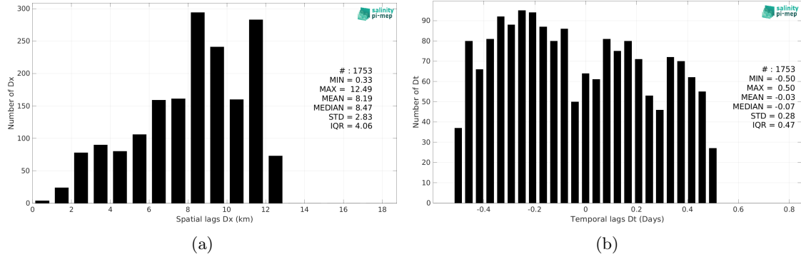
Figure 5: Histograms of the spatial (a) and temporal (b) lags between the location/time of the TSG (SAMOS) measurement and the date of the corresponding SMOS SSS L2Q v331 - 0.25 Deg (CATDS-CPDC) SSS pixel.
