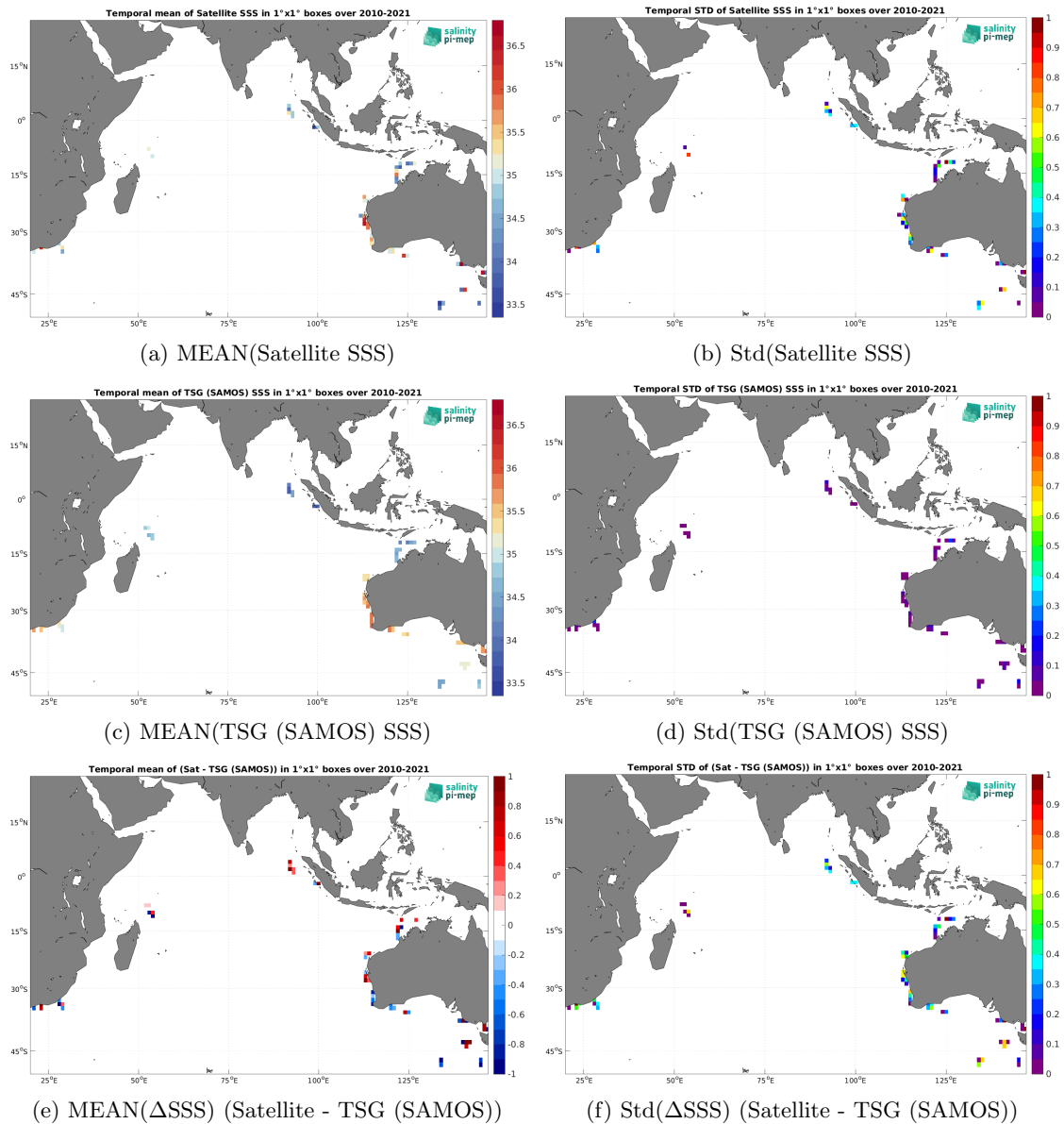
Figure 6: Temporal mean (left) and Std (right) of SSS from SMOS SSS L2Q v331 - 0.25 Deg (CATDS-CPDC) (top), TSG (SAMOS) (middle), and of \Delta SSS (Satellite - TSG (SAMOS)). Only match-up pairs are used to generate these maps.
