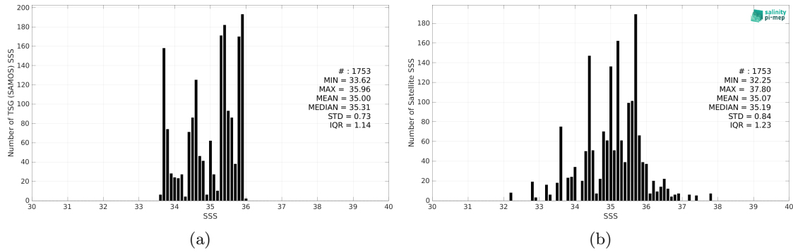
Figure 2: Histograms of SSS from TSG (SAMOS) (a) and SMOS SSS L2Q v331 - 0.25 Deg (CATDS-CPDC) (b) considering all match-up pairs per bins of 0.1 over the Indian Ocean Pi-MEP region and for the full satellite product period.
