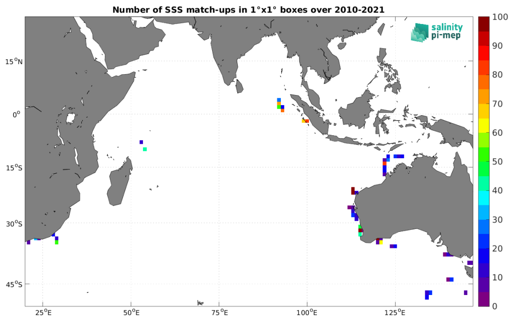
Figure 4: Number of SSS match-ups between TSG (SAMOS) SSS and the SMOS SSS L2Q v331 - 0.25 Deg (CATDS-CPDC) SSS product for the Indian Ocean Pi-MEP region over 1^\circ \times 1^\circ boxes and for the full satellite product period.
