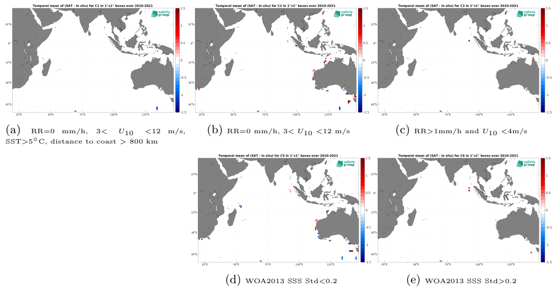
Figure 12: Temporal mean gridded over spatial boxes of size 1^\circ \times 1^\circ of \Delta SSS (SMOS SSS L2Q v331 - 0.25 Deg (CATDS-CPDC) - TSG (SAMOS)) for 5 different subdatasets corresponding to:RR=0 mm/h, 3 < U_{10} < 12 m/s, SST >5^\circ C, distance to coast > 800 km (a), RR=0 mm/h, 3 < U_{10} < 12 m/s (b), RR >1 mm/h and U_{10} < 4 m/s (c), WOA2013 SSS Std <0.2 (d), WOA2013 SSS Std >0.2 (e).
