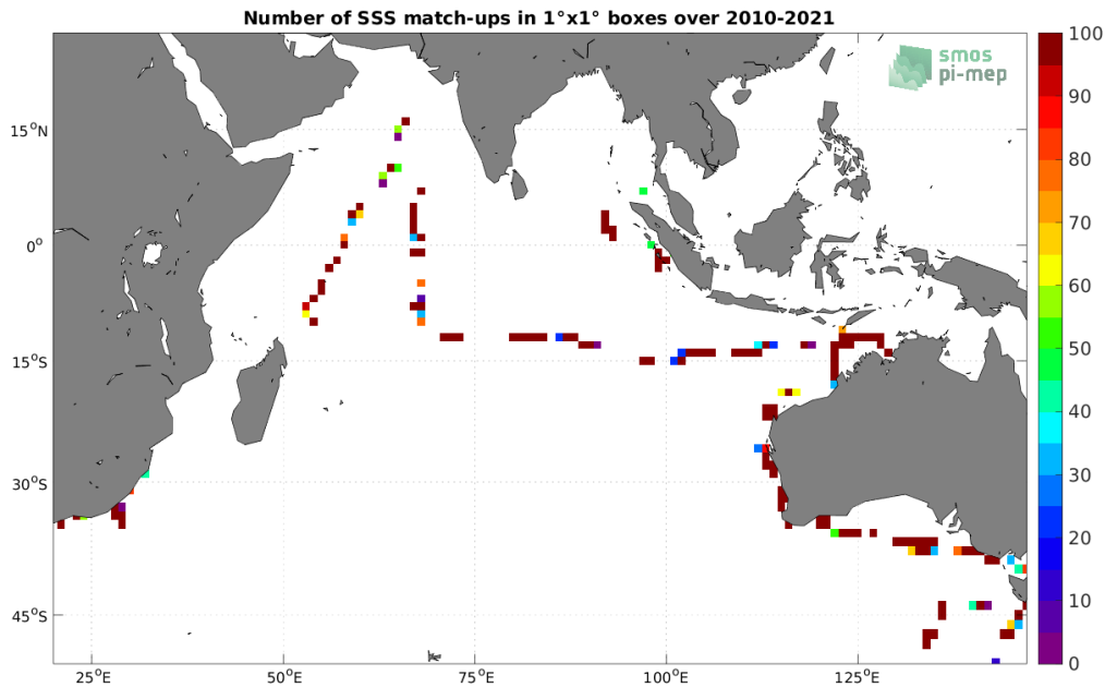
Figure 4: Number of SSS match-ups between TSG (SAMOS) SSS and the SMOS SSS L2Q v331 - 0.25 Deg (CATDS-CPDC) SSS product for the Indian Ocean Pi-MEP region over 1^\circ \times 1^\circ boxes and for the full satellite product period.
