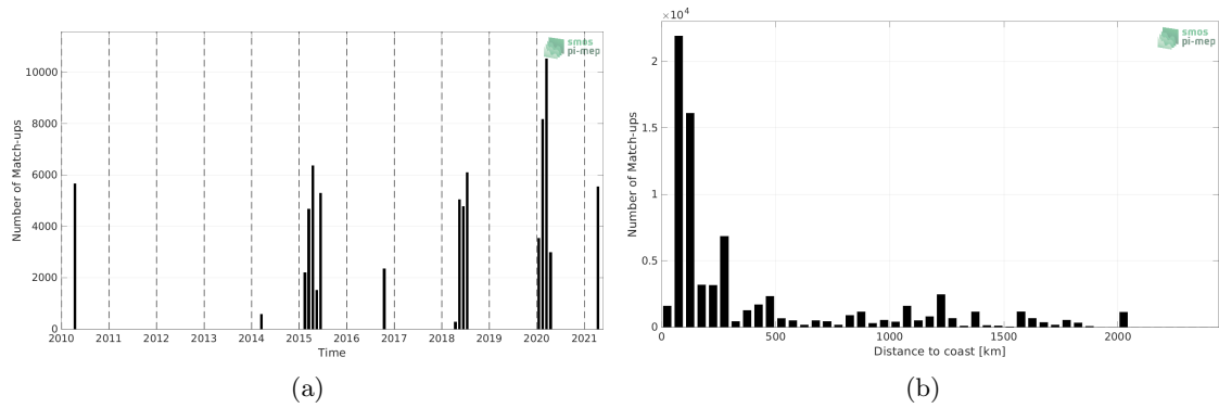
Figure 1: Number of match-ups between TSG (SAMOS) and SMOS SSS L2Q v331 - 0.25 Deg (CATDS-CPDC) SSS as a function of time (a) and as function of the distance to coast (b) over the Indian Ocean Pi-MEP region and for the full satellite product period.
