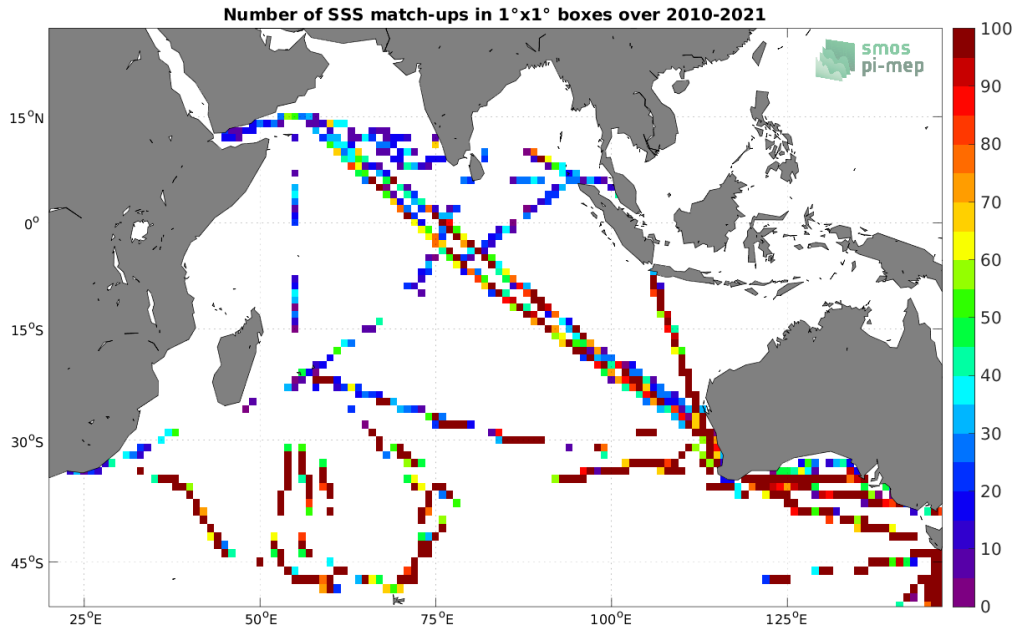
Figure 4: Number of SSS match-ups between TSG (LEGOS-DM) SSS and the SMOS SSS L2Q v331 - 0.25 Deg (CATDS-CPDC) SSS product for the Indian Ocean Pi-MEP region over 1^\circ \times 1^\circ boxes and for the full satellite product period.
