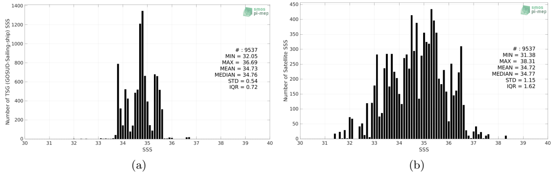
Figure 2: Histograms of SSS from TSG (GOSUD-Sailing-ship) (a) and SMOS SSS L2Q v331 - 0.25 Deg (CATDS-CPDC) (b) considering all match-up pairs per bins of 0.1 over the Indian Ocean Pi-MEP region and for the full satellite product period.
