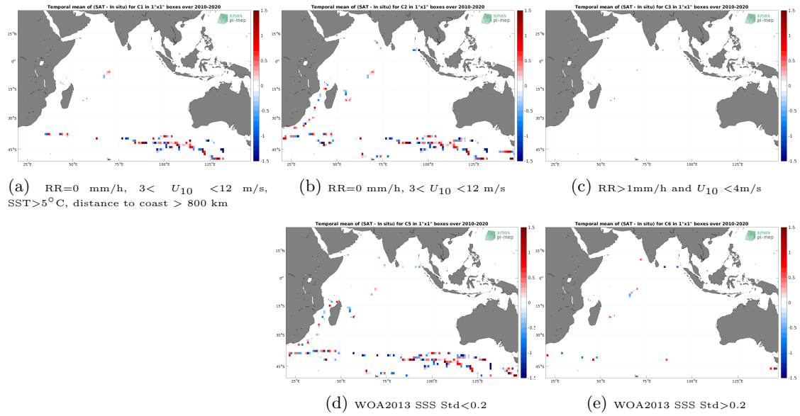
Figure 12: Temporal mean gridded over spatial boxes of size 1^\circ \times 1^\circ of \Delta SSS (SMOS SSS L2Q v331 - 0.25 Deg (CATDS-CPDC) - TSG (GOSUD-Sailing-ship)) for 5 different subdatasets corresponding to: RR=0 mm/h, 3 < U_{10} < 12 m/s, SST > 5^\circ\text{C} , distance to coast > 800 km (a), RR=0 mm/h, 3 < U_{10} < 12 m/s (b), RR > 1 mm/h and U_{10} < 4 m/s (c), WOA2013 SSS Std < 0.2 (d), WOA2013 SSS Std > 0.2 (e).
