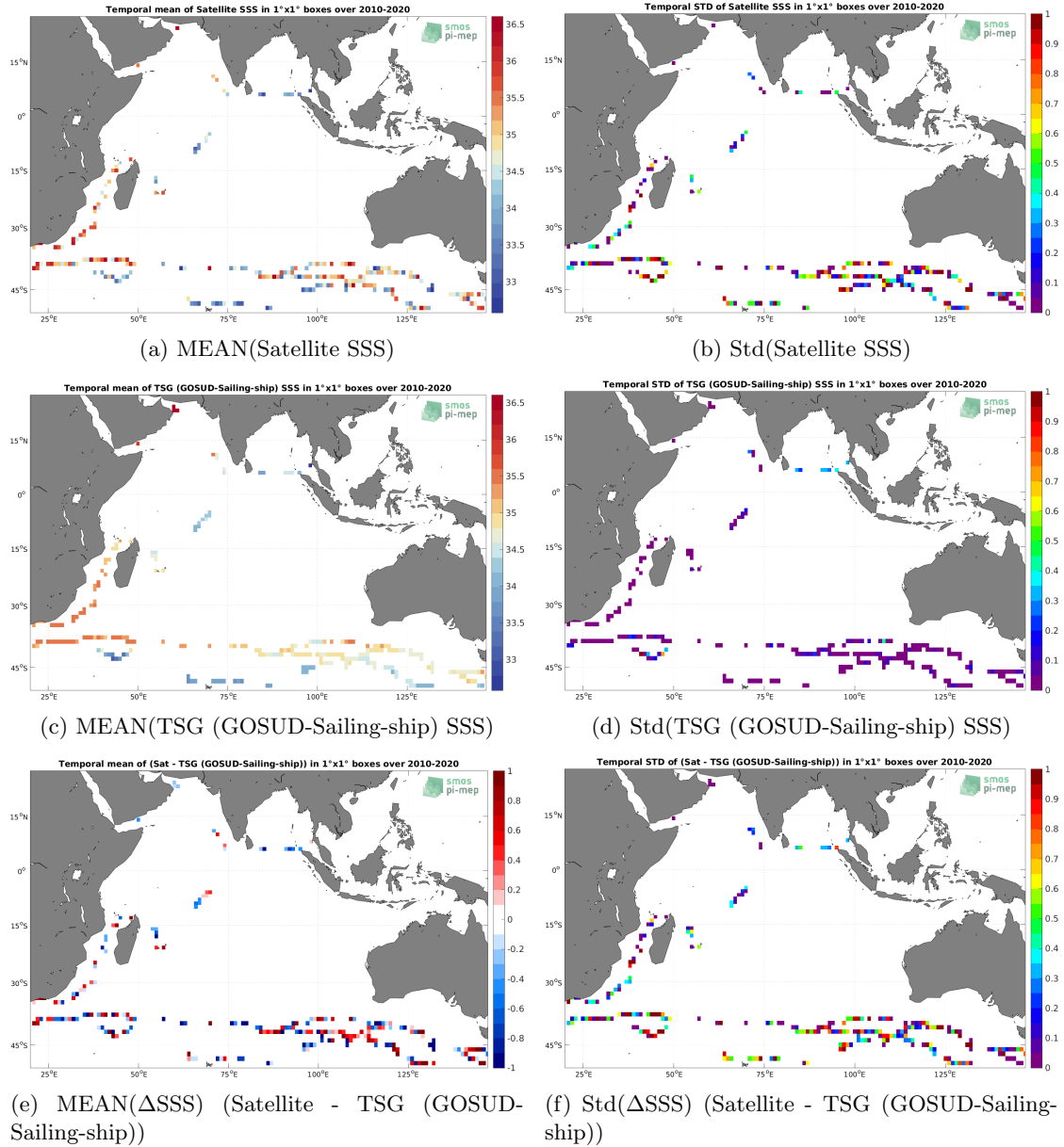
Figure 6: Temporal mean (left) and Std (right) of SSS from SMOS SSS L2Q v331 - 0.25 Deg (CATDS-CPDC) (top), TSG (GOSUD-Sailing-ship) (middle), and of \Delta SSS (Satellite - TSG (GOSUD-Sailing-ship)). Only match-up pairs are used to generate these maps.
