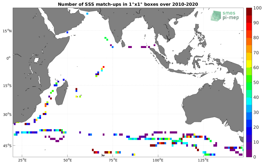
Figure 4: Number of SSS match-ups between TSG (GOSUD-Sailing-ship) SSS and the SMOS SSS L2Q v331 - 0.25 Deg (CATDS-CPDC) SSS product for the Indian Ocean Pi-MEP region over 1^\circ \times 1^\circ boxes and for the full satellite product period.
