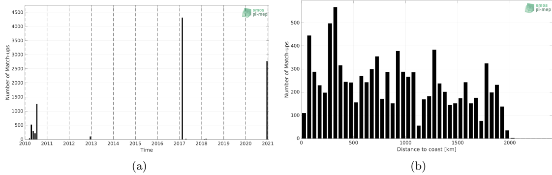
Figure 1: Number of match-ups between TSG (GOSUD-Sailing-ship) and SMOS SSS L2Q v331 - 0.25 Deg (CATDS-CPDC) SSS as a function of time (a) and as function of the distance to coast (b) over the Indian Ocean Pi-MEP region and for the full satellite product period.
