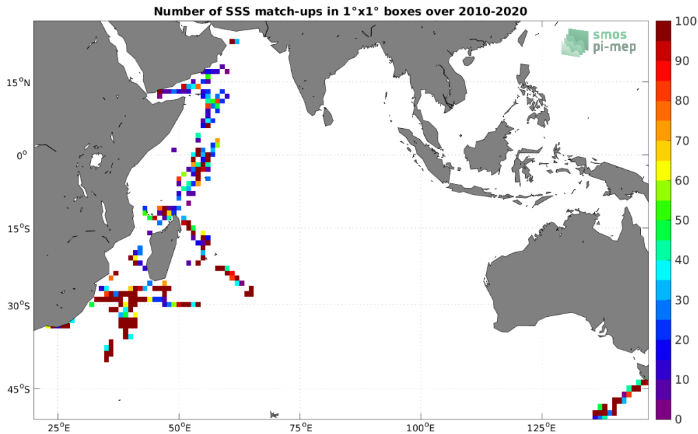
Figure 4: Number of SSS match-ups between TSG (GOSUD-Research-vessel) SSS and the SMOS SSS L2Q v331 - 0.25 Deg (CATDS-CPDC) SSS product for the Indian Ocean Pi-MEP region over 1^\circ \times 1^\circ boxes and for the full satellite product period.
