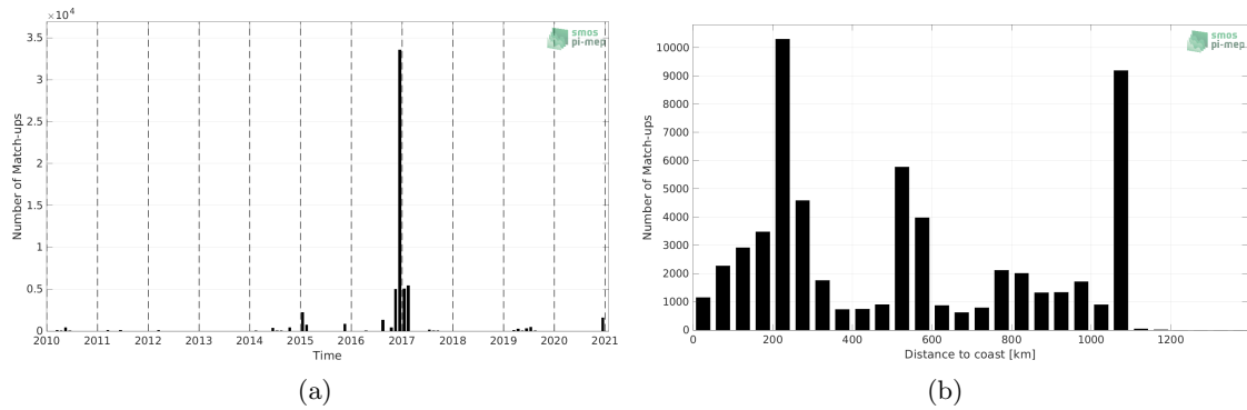
Figure 1: Number of match-ups between TSG (GOSUD-Research-vessel) and SMOS SSS L2Q v331 - 0.25 Deg (CATDS-CPDC) SSS as a function of time (a) and as function of the distance to coast (b) over the Indian Ocean Pi-MEP region and for the full satellite product period.
