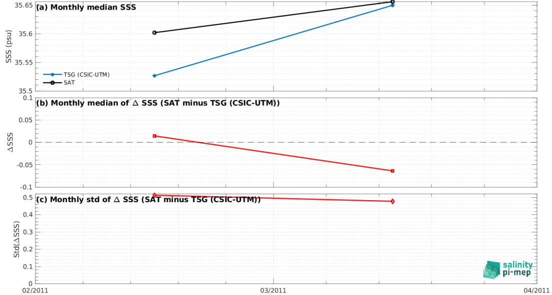
Figure 7: Time series of the monthly median SSS (top), median of \Delta SSS (Satellite - TSG (CSIC-UTM)) and Std of \Delta SSS (Satellite - TSG (CSIC-UTM)) over the Indian Ocean Pi-MEP region considering all match-ups collected by the Pi-MEP.
