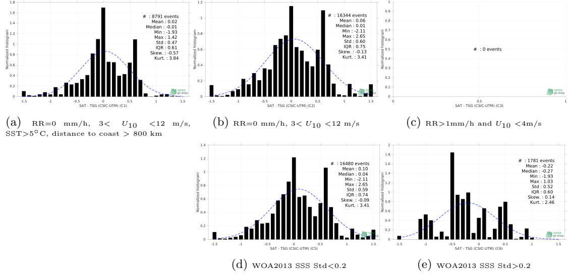
Figure 13: Normalized histogram of \Delta SSS (SMOS SSS L2Q v331 - 0.25 Deg (CATDS-CPDC) - TSG (CSIC-UTM)) for 5 different subdatasets corresponding to: RR=0 mm/h, 3 < U_{10} < 12 m/s, SST>5°C, distance to coast > 800 km (a), RR=0 mm/h, 3 < U_{10} < 12 m/s (b), RR>1mm/h and U_{10} < 4 m/s (c), WOA2013 SSS Std<0.2 (d), WOA2013 SSS Std>0.2 (e).
