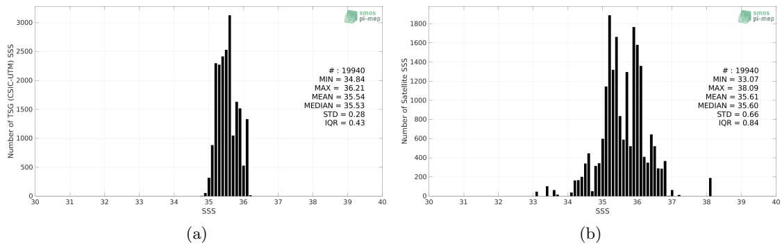
Figure 2: Histograms of SSS from TSG (CSIC-UTM) (a) and SMOS SSS L2Q v331 - 0.25 Deg (CATDS-CPDC) (b) considering all match-up pairs per bins of 0.1 over the Indian Ocean Pi-MEP region and for the full satellite product period.
