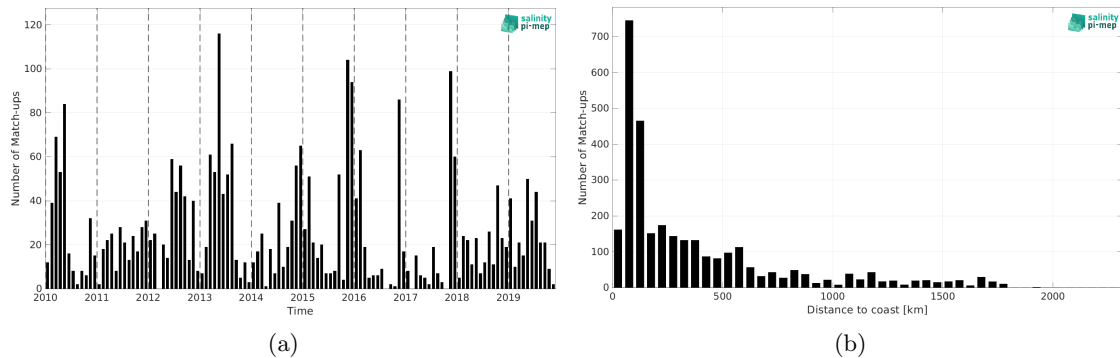
Figure 1: Number of match-ups between Marine mammals and SMOS SSS L2Q v331 - 0.25 Deg (CATDS-CPDC) SSS as a function of time (a) and as function of the distance to coast (b) over the Indian Ocean Pi-MEP region and for the full satellite product period.
