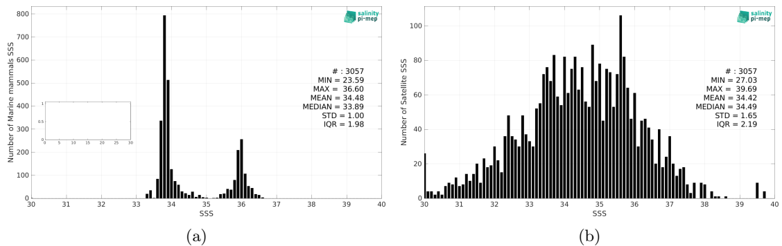
Figure 2: Histograms of SSS from Marine mammals (a) and SMOS SSS L2Q v331 - 0.25 Deg (CATDS-CPDC) (b) considering all match-up pairs per bins of 0.1 over the Indian Ocean Pi-MEP region and for the full satellite product period.
