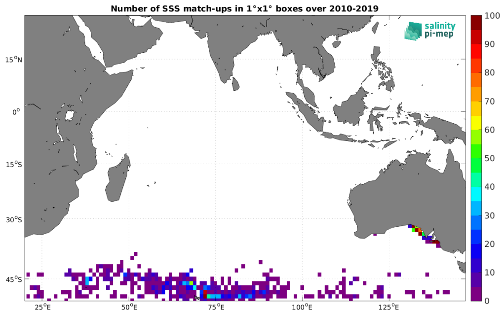
Figure 4: Number of SSS match-ups between Marine mammals SSS and the SMOS SSS L2Q v331 - 0.25 Deg (CATDS-CPDC) SSS product for the Indian Ocean Pi-MEP region over 1^\circ \times 1^\circ boxes and for the full satellite product period.
