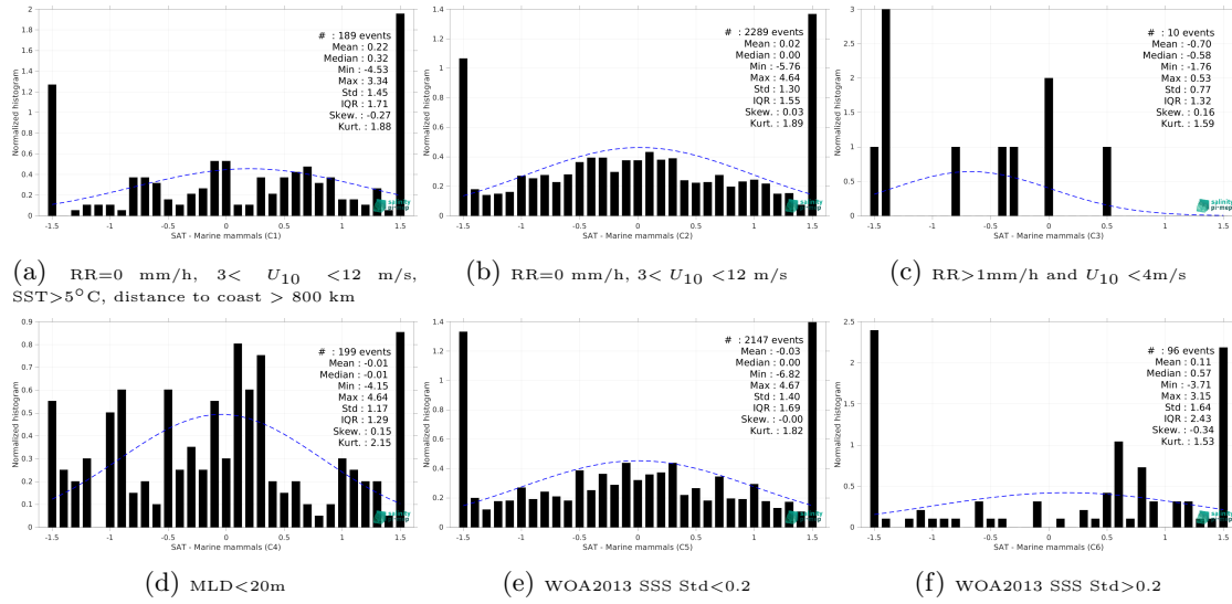
Figure 13: Normalized histogram of \Delta SSS (SMOS SSS L2Q v331 - 0.25 Deg (CATDS-CPDC) - Marine mammals) for 6 different subdatasets corresponding to: RR=0 mm/h, 3 < U_{10} < 12 m/s, SST>5°C, distance to coast > 800 km (a), RR=0 mm/h, 3 < U_{10} < 12 m/s (b), RR>1mm/h and U_{10} < 4 m/s (c), MLD<20m (d), WOA2013 SSS Std<0.2 (e), WOA2013 SSS Std>0.2 (f).
