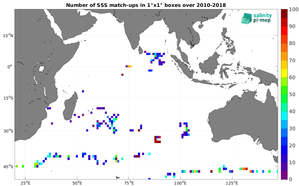
Figure 3: Number of SSS match-ups between Surface drifters SSS and the SMOS SSS L2Q v331 - 0.25 Deg (CATDS-CPDC) SSS product for the Indian Ocean Pi-MEP region over 1^\circ \times 1^\circ boxes and for the full satellite product period.
