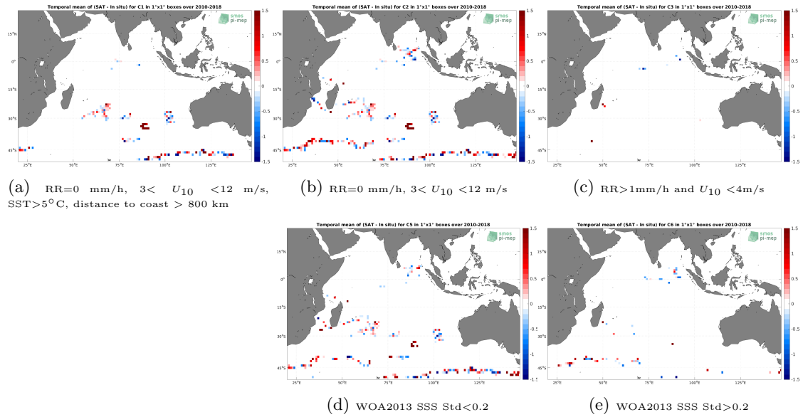
Figure 11: Temporal mean gridded over spatial boxes of size 1^\circ \times 1^\circ of \Delta SSS (SMOS SSS L2Q v331 - 0.25 Deg (CATDS-CPDC) - Surface drifters) for 5 different subdatasets corresponding to:RR=0 mm/h, 3 < U_{10} < 12 m/s, SST >5^\circ C, distance to coast > 800 km (a), RR=0 mm/h, 3 < U_{10} < 12 m/s (b), RR >1 mm/h and U_{10} < 4 m/s (c), WOA2013 SSS Std <0.2 (d), WOA2013 SSS Std >0.2 (e).
