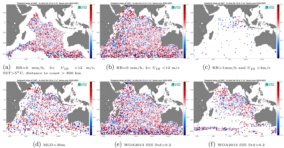
Figure 12: Temporal mean gridded over spatial boxes of size 1^\circ \times 1^\circ of \Delta SSS (SMOS SSS L2Q v331 - 0.25 Deg (CATDS-CPDC) - Argo) for 6 different subdatasets corresponding to:RR=0 mm/h, 3 < U_{10} < 12 m/s, SST >5^\circ C, distance to coast > 800 km (a), RR=0 mm/h, 3 < U_{10} < 12 m/s (b), RR >1 mm/h and U_{10} < 4 m/s (c),MLD <20 m (d),WOA2013 SSS Std <0.2 (e),WOA2013 SSS Std >0.2 (f).
