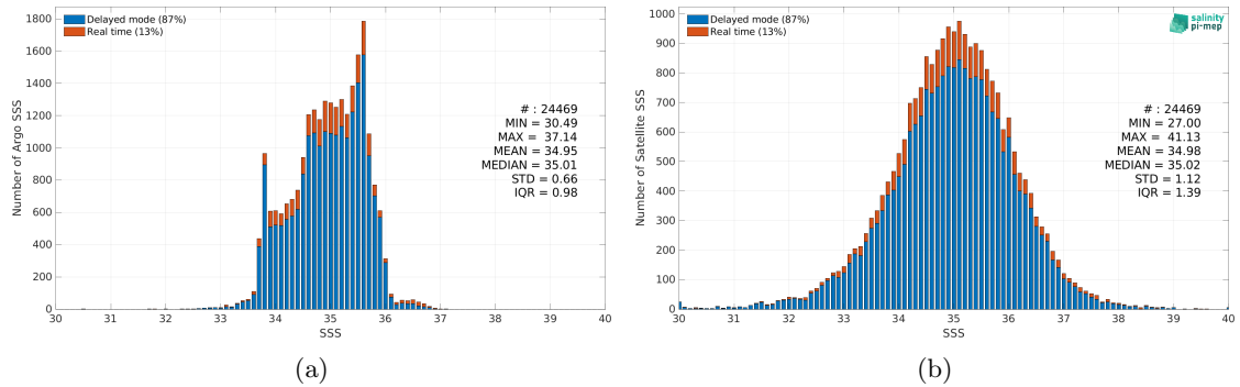
Figure 2: Histograms of SSS from Argo (a) and SMOS SSS L2Q v331 - 0.25 Deg (CATDS-CPDC) (b) considering all match-up pairs per bins of 0.1 over the Indian Ocean Pi-MEP region and for the full satellite product period.
