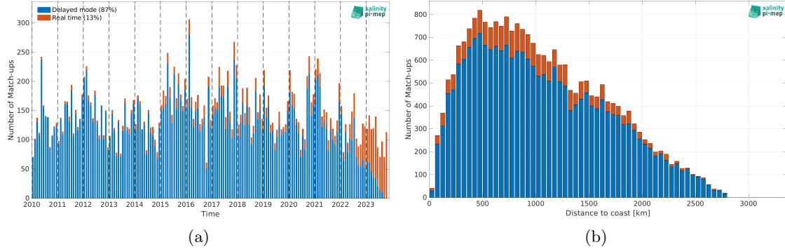
Figure 1: Number of match-ups between Argo and SMOS SSS L2Q v331 - 0.25 Deg (CATDS-CPDC) SSS as a function of time (a) and as function of the distance to coast (b) over the Indian Ocean Pi-MEP region and for the full satellite product period.
