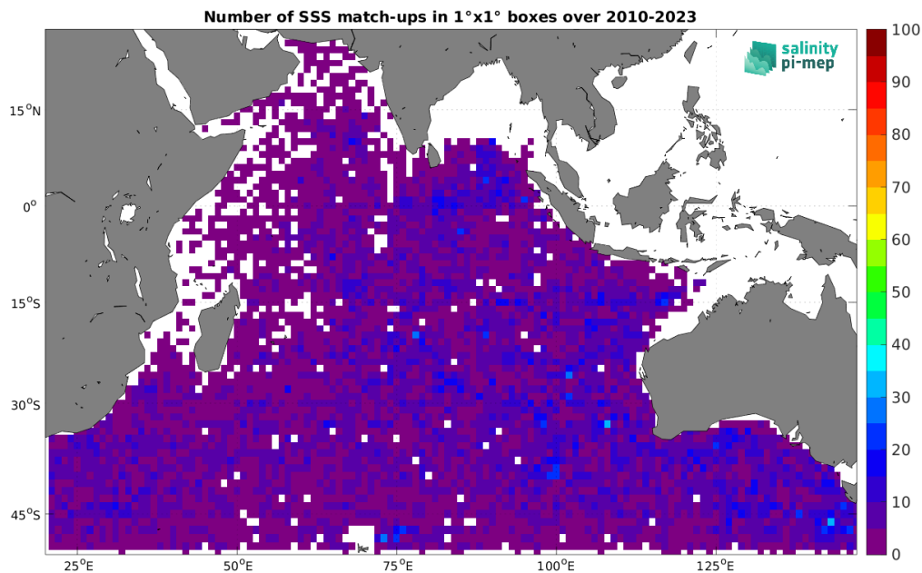
Figure 4: Number of SSS match-ups between Argo SSS and the SMOS SSS L2Q v331 - 0.25 Deg (CATDS-CPDC) SSS product for the Indian Ocean Pi-MEP region over 1^\circ \times 1^\circ boxes and for the full satellite product period.
