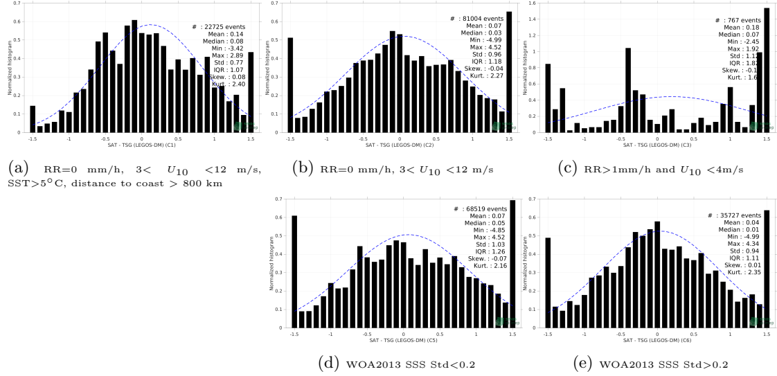
Figure 13: Normalized histogram of \Delta\text{SSS} (SMOS SSS L2Q v330 - 0.25 Deg (CATDS-CPDC) - TSG (LEGOS-DM)) for 5 different subdatasets corresponding to: RR=0 mm/h, 3 < U_{10} < 12 m/s, SST>5°C, distance to coast > 800 km (a), RR=0 mm/h, 3 < U_{10} < 12 m/s (b), RR>1mm/h and U_{10} < 4 m/s (c), WOA2013 SSS Std<0.2 (d), WOA2013 SSS Std>0.2 (e).
