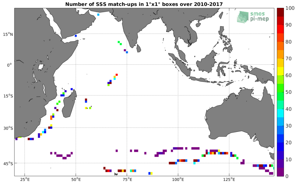
Figure 4: Number of SSS match-ups between TSG (GOSUD-Sailing-ship) SSS and the SMOS SSS L2Q v330 - 0.25 Deg (CATDS-CPDC) SSS product for the Indian Ocean Pi-MEP region over 1^\circ \times 1^\circ boxes and for the full satellite product period.
