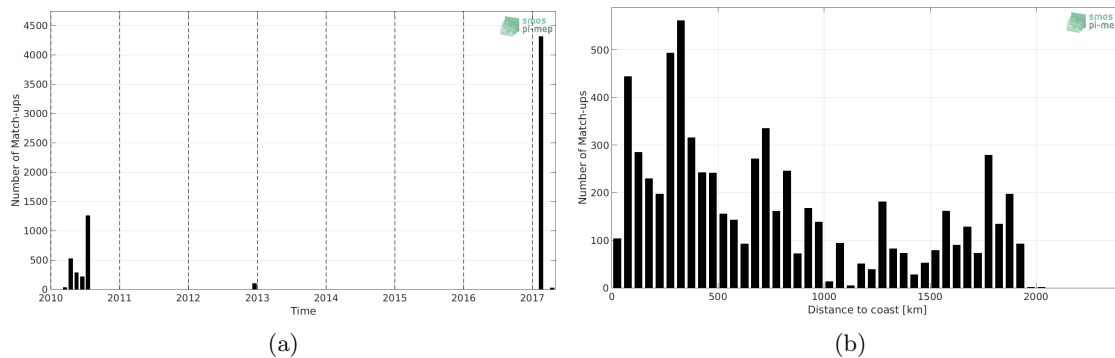
Figure 1: Number of match-ups between TSG (GOSUD-Sailing-ship) and SMOS SSS L2Q v330 - 0.25 Deg (CATDS-CPDC) SSS as a function of time (a) and as function of the distance to coast (b) over the Indian Ocean Pi-MEP region and for the full satellite product period.
