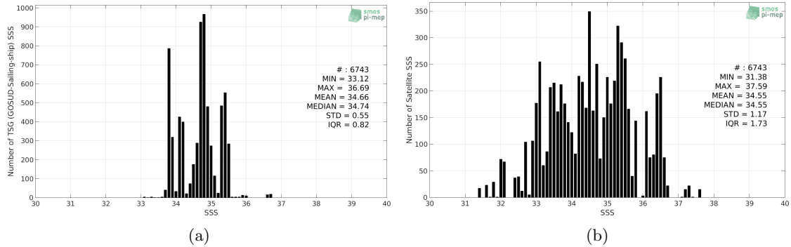
Figure 2: Histograms of SSS from TSG (GOSUD-Sailing-ship) (a) and SMOS SSS L2Q v330 - 0.25 Deg (CATDS-CPDC) (b) considering all match-up pairs per bins of 0.1 over the Indian Ocean Pi-MEP region and for the full satellite product period.
