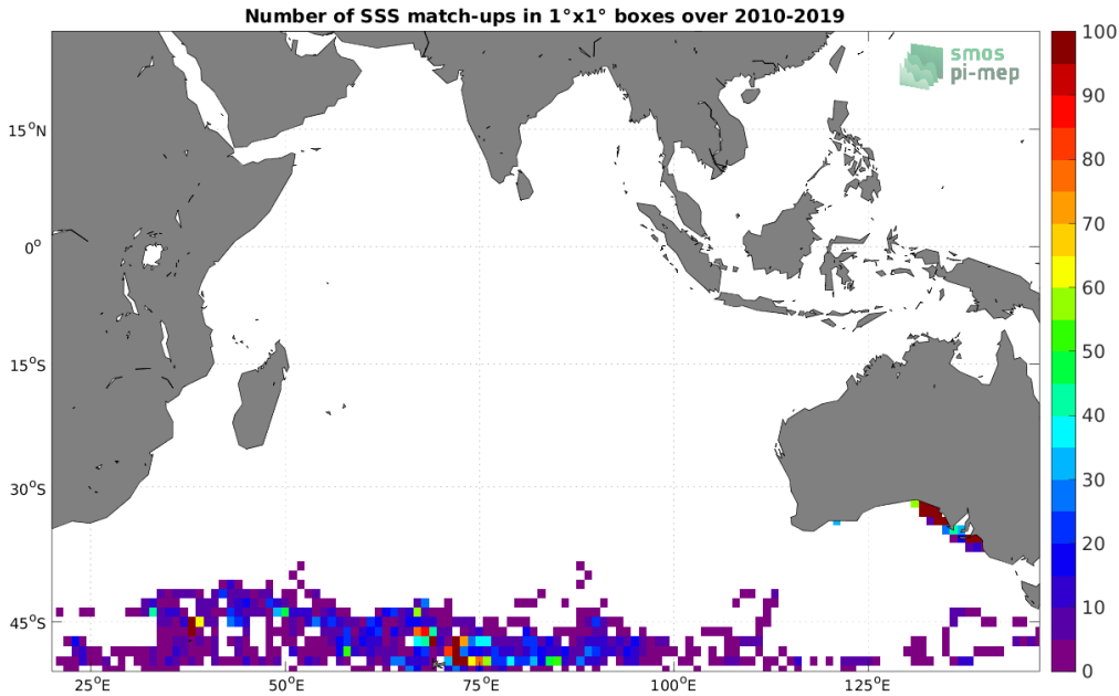
Figure 4: Number of SSS match-ups between Marine mammals SSS and the SMOS SSS L2Q v330 - 0.25 Deg (CATDS-CPDC) SSS product for the Indian Ocean Pi-MEP region over 1^\circ \times 1^\circ boxes and for the full satellite product period.
