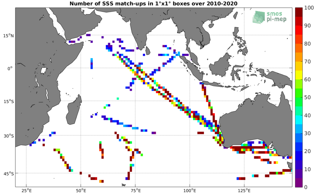
Figure 4: Number of SSS match-ups between TSG (LEGOS-DM) SSS and the SMOS SSS L2Q v321 - 0.25 Deg (CATDS-CPDC) SSS product for the Indian Ocean Pi-MEP region over 1^\circ \times 1^\circ boxes and for the full satellite product period.
