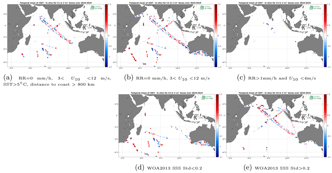
Figure 12: Temporal mean gridded over spatial boxes of size 1^\circ \times 1^\circ of \Delta SSS (SMOS SSS L2Q v321 - 0.25 Deg (CATDS-CPDC) - TSG (LEGOS-DM)) for 5 different subdatasets corresponding to: RR=0 mm/h, 3 < U_{10} < 12 m/s, SST >5^\circ C, distance to coast > 800 km (a), RR=0 mm/h, 3 < U_{10} < 12 m/s (b), RR >1 mm/h and U_{10} < 4 m/s (c), WOA2013 SSS Std <0.2 (d), WOA2013 SSS Std >0.2 (e).
