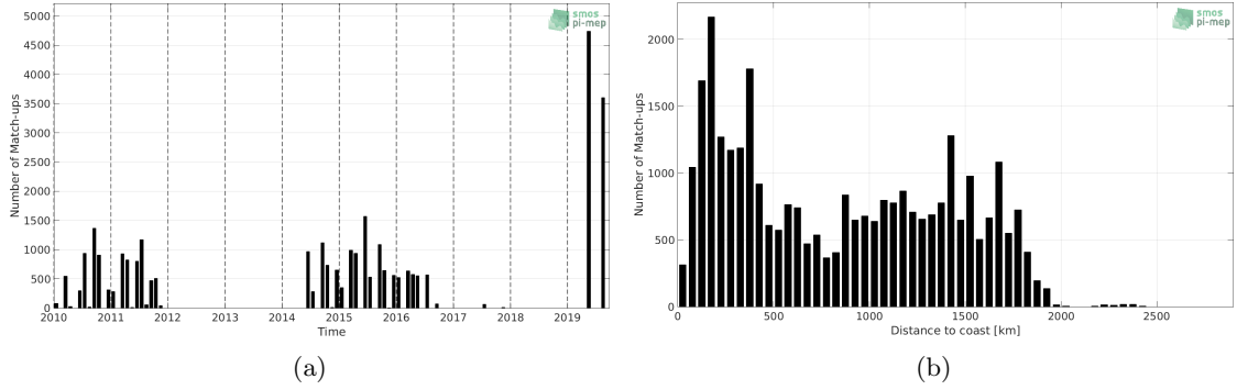
Figure 1: Number of match-ups between TSG (LEGOS-DM) and SMOS SSS L2Q v321 - 0.25 Deg (CATDS-CPDC) SSS as a function of time (a) and as function of the distance to coast (b) over the Indian Ocean Pi-MEP region and for the full satellite product period.
