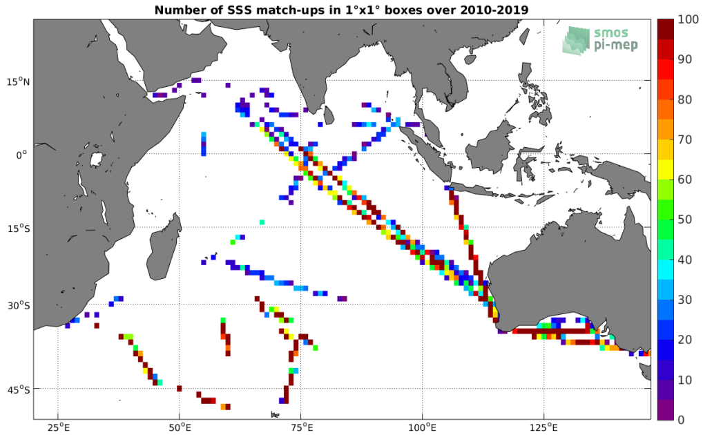
Figure 4: Number of SSS match-ups between TSG (LEGOS-DM) SSS and the SMOS SSS L2Q v321 - 0.25 Deg (CATDS-CPDC) SSS product for the Indian Ocean Pi-MEP region over 1°x1° boxes and for the full satellite product period.
