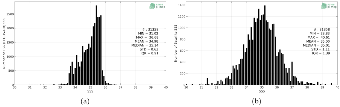
Figure 2: Histograms of SSS from TSG (LEGOS-DM) (a) and SMOS SSS L2Q v321 - 0.25 Deg (CATDS-CPDC) (b) considering all match-up pairs per bins of 0.1 over the Indian Ocean Pi-MEP region and for the full satellite product period.
