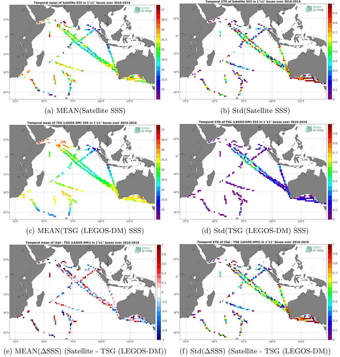
Figure 6: Temporal mean (left) and Std (right) of SSS from SMOS SSS L2Q v321 - 0.25 Deg (CATDS-CPDC) (top), TSG (LEGOS-DM) (middle), and of \Delta SSS (Satellite - TSG (LEGOS-DM)). Only match-up pairs are used to generate these maps.
