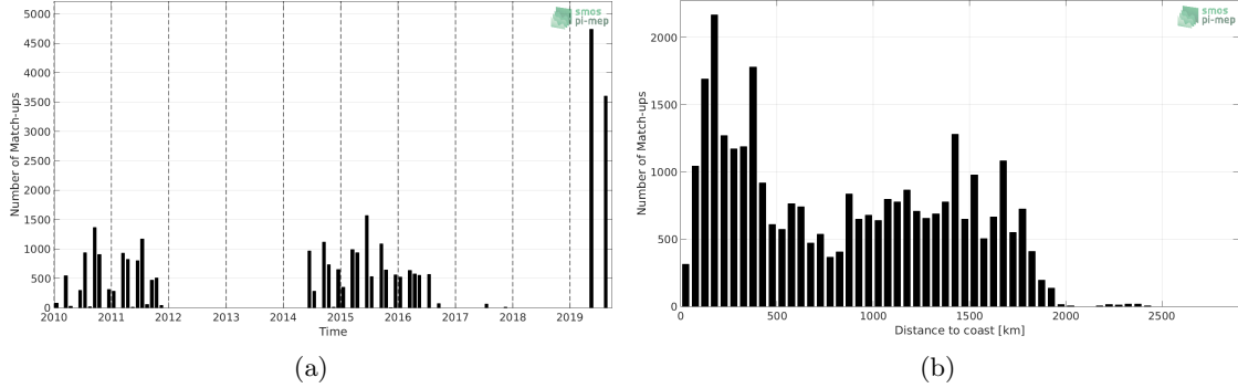
Figure 1: Number of match-ups between TSG-LEGOS-DM and SMOS L2Q v321 - 0.25 Deg (CATDS-CPDC) SSS as a function of time (a) and as function of the distance to coast (b) over the Indian Ocean Pi-MEP region and for the full satellite product period.
