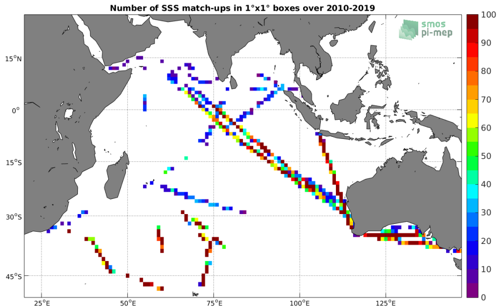
Figure 4: Number of SSS match-ups between TSG-LEGOS-DM SSS and the SMOS L2Q v321 - 0.25 Deg (CATDS-CPDC) SSS product for the Indian Ocean Pi-MEP region over 1°x1° boxes and for the full satellite product period.
