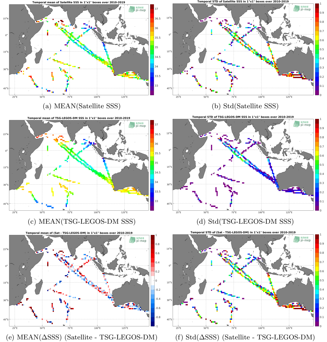
Figure 6: Temporal mean (left) and Std (right) of SSS from SMOS L2Q v321 - 0.25 Deg (CATDS-CPDC) (top), TSG-LEGOS-DM (middle), and of \Delta SSS (Satellite - TSG-LEGOS-DM). Only match-up pairs are used to generate these maps.
