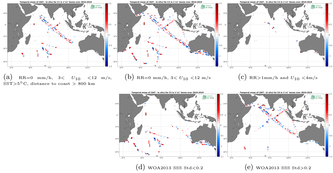
Figure 12: Temporal mean gridded over spatial boxes of size 1^\circ \times 1^\circ of \Delta SSS (SMOS L2Q v321 - 0.25 Deg (CATDS-CPDC) - TSG-LEGOS-DM) for 5 different subdatasets corresponding to: RR=0 mm/h, 3 < U_{10} < 12 m/s, SST > 5^\circ C , distance to coast > 800 km (a), RR=0 mm/h, 3 < U_{10} < 12 m/s (b), RR > 1 mm/h and U_{10} < 4 m/s (c), WOA2013 SSS Std < 0.2 (d), WOA2013 SSS Std > 0.2 (e).
