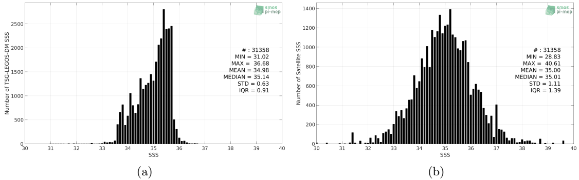
Figure 2: Histograms of SSS from TSG-LEGOS-DM (a) and SMOS L2Q v321 - 0.25 Deg (CATDS-CPDC) (b) considering all match-up pairs per bins of 0.1 over the Indian Ocean Pi-MEP region and for the full satellite product period.
