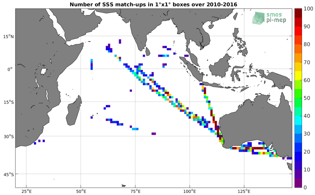
Figure 4: Number of SSS match-ups between TSG-LEGOS-DM SSS and the SMOS-L3-CATDS-CPDC-V321-L2Q SSS product for the Indian Ocean Pi-MEP region over 1°x1° boxes and for the full satellite product period.
