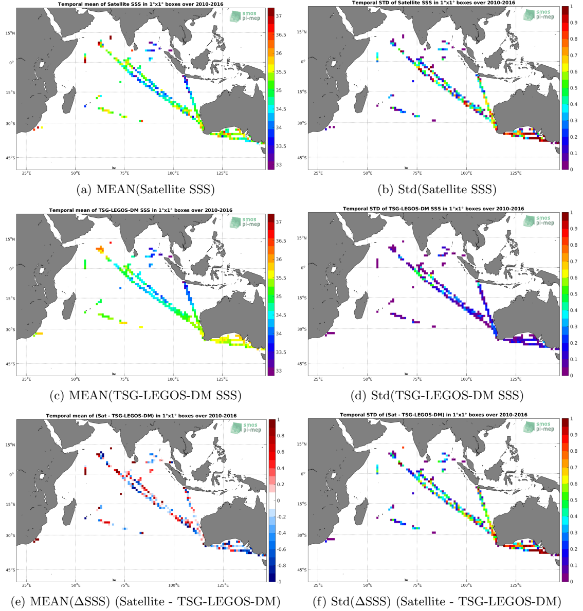
Figure 6: Temporal mean (left) and Std (right) of SSS from SMOS-L3-CATDS-CPDC-V321-L2Q (top), TSG-LEGOS-DM (middle), and of \Delta SSS (Satellite - TSG-LEGOS-DM). Only match-up pairs are used to generate these maps.
