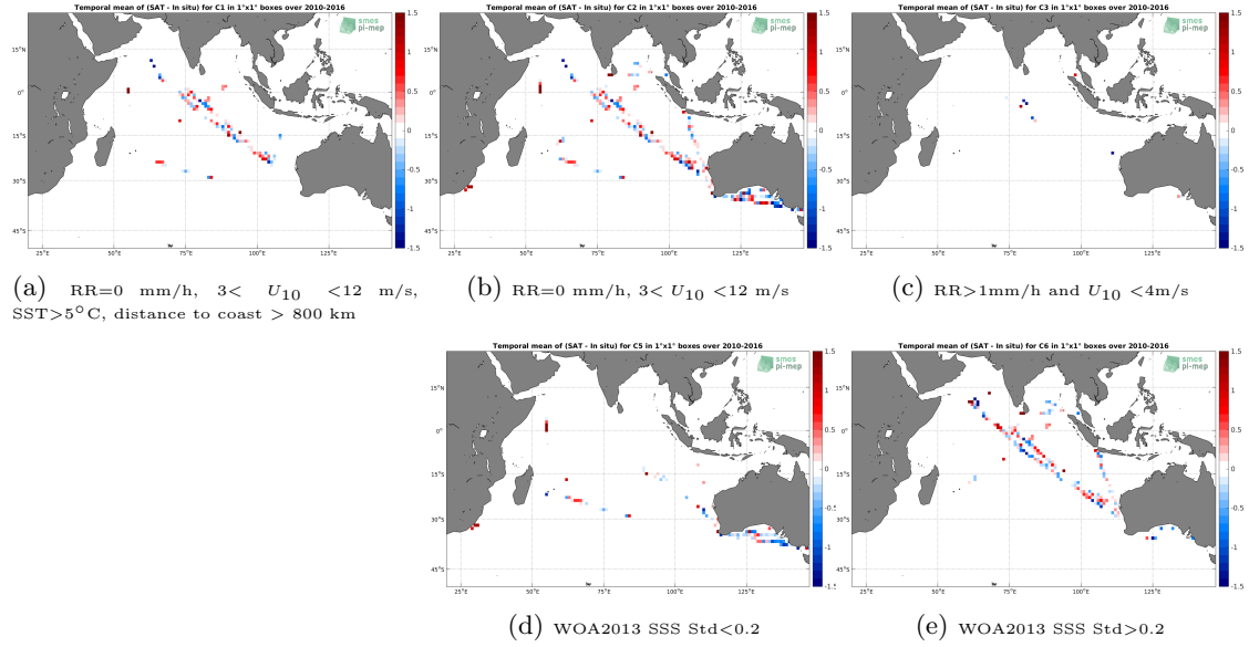
Figure 12: Temporal mean gridded over spatial boxes of size 1^\circ \times 1^\circ of \Delta SSS (SMOS-L3-CATDS-CPDC-V321-L2Q - TSG-LEGOS-DM) for 5 different subdatasets corresponding to: RR=0 mm/h, 3 < U_{10} < 12 m/s, SST > 5^\circ C , distance to coast > 800 km (a), RR=0 mm/h, 3 < U_{10} < 12 m/s (b), RR > 1 mm/h and U_{10} < 4 m/s (c), WOA2013 SSS Std < 0.2 (d), WOA2013 SSS Std > 0.2 (e).
