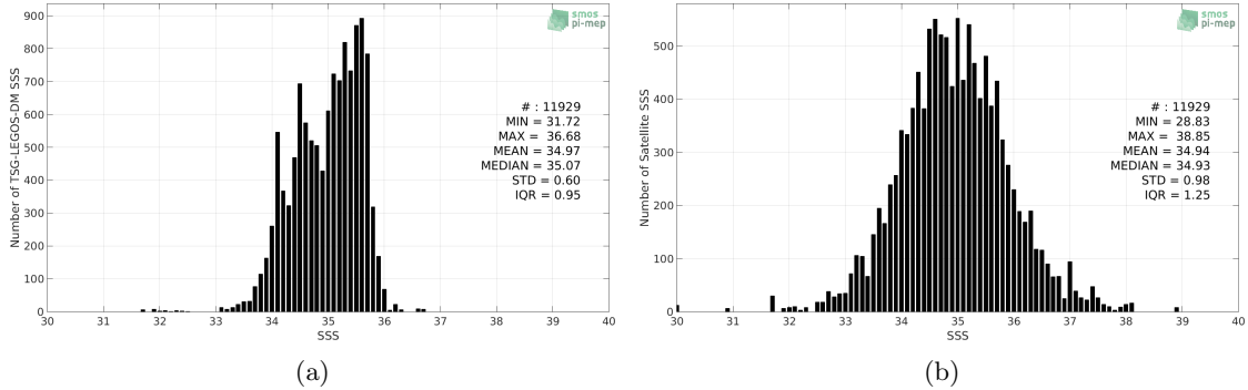
Figure 2: Histograms of SSS from TSG-LEGOS-DM (a) and SMOS-L3-CATDS-CPDC-V321-L2Q (b) considering all match-up pairs per bins of 0.1 over the Indian Ocean Pi-MEP region and for the full satellite product period.
