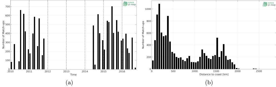
Figure 1: Number of match-ups between TSG-LEGOS-DM and SMOS-L3-CATDS-CPDC-V321-L2Q SSS as a function of time (a) and as function of the distance to coast (b) over the Indian Ocean Pi-MEP region and for the full satellite product period.
