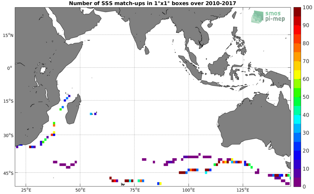
Figure 4: Number of SSS match-ups between TSG (GOSUD-Sailing-ship) SSS and the SMOS SSS L2Q v321 - 0.25 Deg (CATDS-CPDC) SSS product for the Indian Ocean Pi-MEP region over 1^\circ \times 1^\circ boxes and for the full satellite product period.
