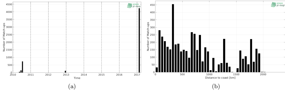
Figure 1: Number of match-ups between TSG (GOSUD-Sailing-ship) and SMOS SSS L2Q v321 - 0.25 Deg (CATDS-CPDC) SSS as a function of time (a) and as function of the distance to coast (b) over the Indian Ocean Pi-MEP region and for the full satellite product period.
