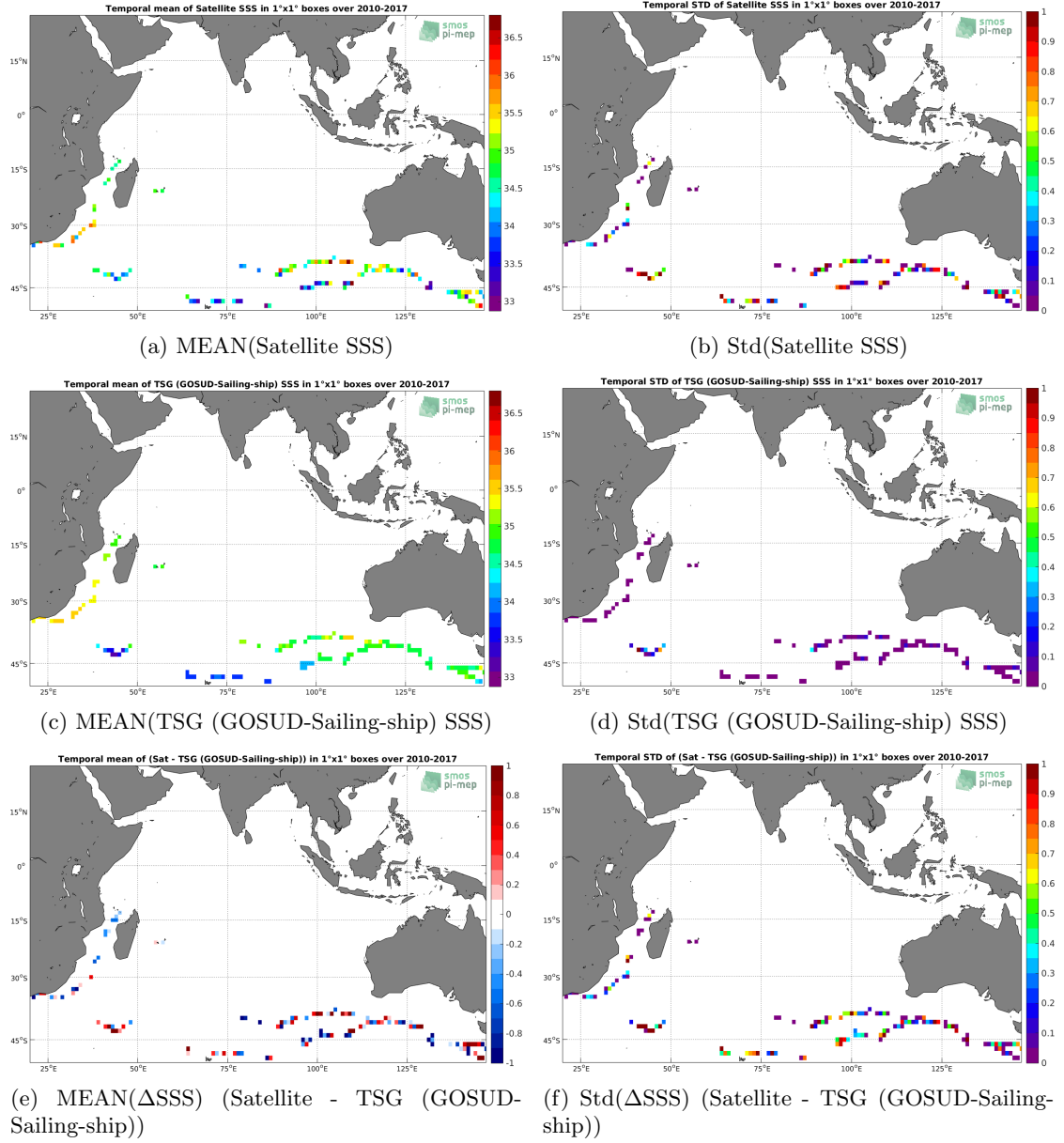
Figure 6: Temporal mean (left) and Std (right) of SSS from SMOS SSS L2Q v321 - 0.25 Deg (CATDS-CPDC) (top), TSG (GOSUD-Sailing-ship) (middle), and of \Delta SSS (Satellite - TSG (GOSUD-Sailing-ship)). Only match-up pairs are used to generate these maps.
