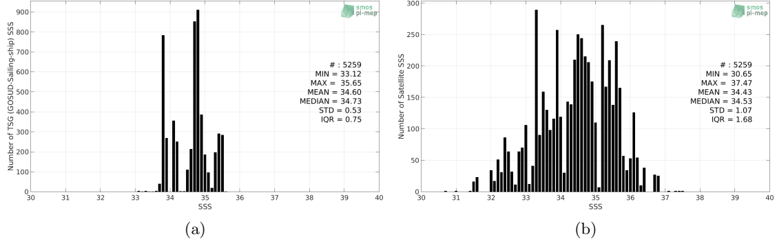
Figure 2: Histograms of SSS from TSG (GOSUD-Sailing-ship) (a) and SMOS SSS L2Q v321 - 0.25 Deg (CATDS-CPDC) (b) considering all match-up pairs per bins of 0.1 over the Indian Ocean Pi-MEP region and for the full satellite product period.
