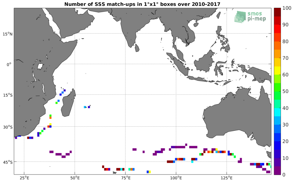
Figure 4: Number of SSS match-ups between TSG (GOSUD-Sailing-ship) SSS and the SMOS SSS L2Q v321 - 0.25 Deg (CATDS-CPDC) SSS product for the Indian Ocean Pi-MEP region over 1°x1° boxes and for the full satellite product period.
