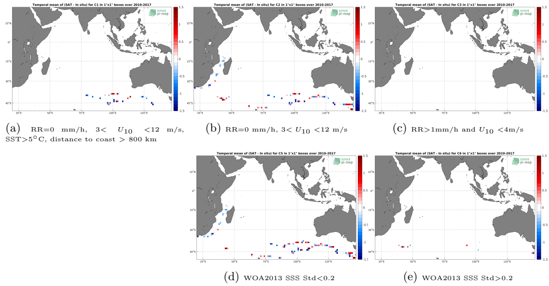
Figure 12: Temporal mean gridded over spatial boxes of size 1^\circ \times 1^\circ of \Delta SSS (SMOS L2Q v321 - 0.25 Deg (CATDS-CPDC) - TSG-GOSUD-Sailing-ship) for 5 different subdatasets corresponding to: RR=0 mm/h, 3 < U_{10} < 12 m/s, SST >5^\circ C, distance to coast > 800 km (a), RR=0 mm/h, 3 < U_{10} < 12 m/s (b), RR >1 mm/h and U_{10} < 4 m/s (c), WOA2013 SSS Std <0.2 (d), WOA2013 SSS Std >0.2 (e).
