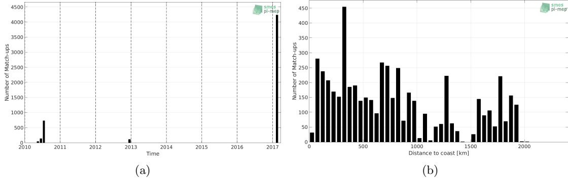
Figure 1: Number of match-ups between TSG-GOSUD-Sailing-ship and SMOS L2Q v321 - 0.25 Deg (CATDS-CPDC) SSS as a function of time (a) and as function of the distance to coast (b) over the Indian Ocean Pi-MEP region and for the full satellite product period.
