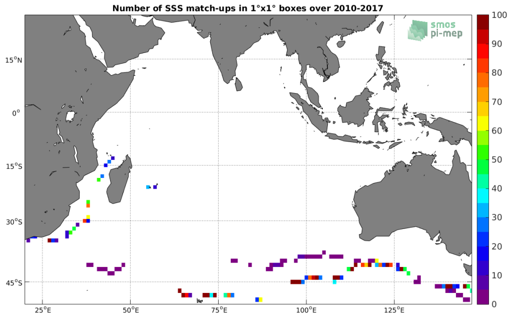
Figure 4: Number of SSS match-ups between TSG-GOSUD-Sailing-ship SSS and the SMOS L2Q v321 - 0.25 Deg (CATDS-CPDC) SSS product for the Indian Ocean Pi-MEP region over 1^\circ \times 1^\circ boxes and for the full satellite product period.
