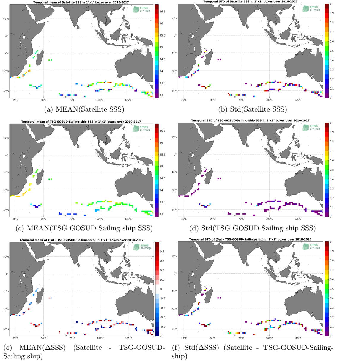
Figure 6: Temporal mean (left) and Std (right) of SSS from SMOS L2Q v321 - 0.25 Deg (CATDS-CPDC) (top), TSG-GOSUD-Sailing-ship (middle), and of \Delta SSS (Satellite - TSG-GOSUD-Sailing-ship). Only match-up pairs are used to generate these maps.
