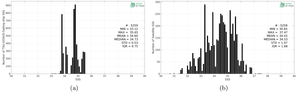
Figure 2: Histograms of SSS from TSG-GOSUD-Sailing-ship (a) and SMOS L2Q v321 - 0.25 Deg (CATDS-CPDC) (b) considering all match-up pairs per bins of 0.1 over the Indian Ocean Pi-MEP region and for the full satellite product period.
