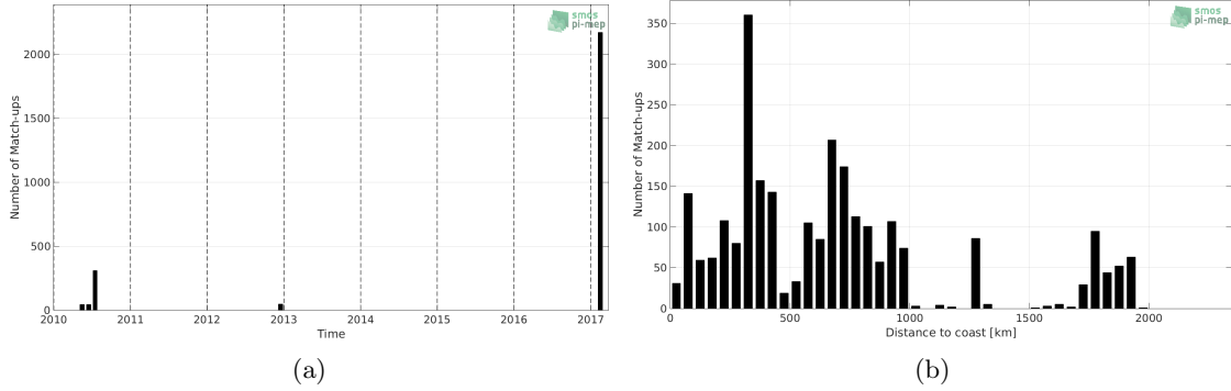
Figure 1: Number of match-ups between TSG-GOSUD-Sailing-ship and SMOS-L3-CATDS-CPDC-V321-L2Q SSS as a function of time (a) and as function of the distance to coast (b) over the Indian Ocean Pi-MEP region and for the full satellite product period.
