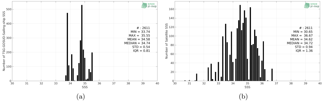
Figure 2: Histograms of SSS from TSG-GOSUD-Sailing-ship (a) and SMOS-L3-CATDS-CPDC-V321-L2Q (b) considering all match-up pairs per bins of 0.1 over the Indian Ocean Pi-MEP region and for the full satellite product period.
