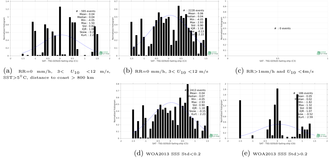
Figure 13: Normalized histogram of \Delta\text{SSS} (SMOS-L3-CATDS-CPDC-V321-L2Q - TSG-GOSUD-Sailing-ship) for 5 different subdatasets corresponding to: RR=0 mm/h, 3 < U_{10} < 12 m/s, SST > 5^\circ\text{C} , distance to coast > 800 km (a), RR=0 mm/h, 3 < U_{10} < 12 m/s (b), RR > 1\text{mm/h} and U_{10} < 4\text{m/s} (c), WOA2013 SSS \text{Std} < 0.2 (d), WOA2013 SSS \text{Std} > 0.2 (e).
