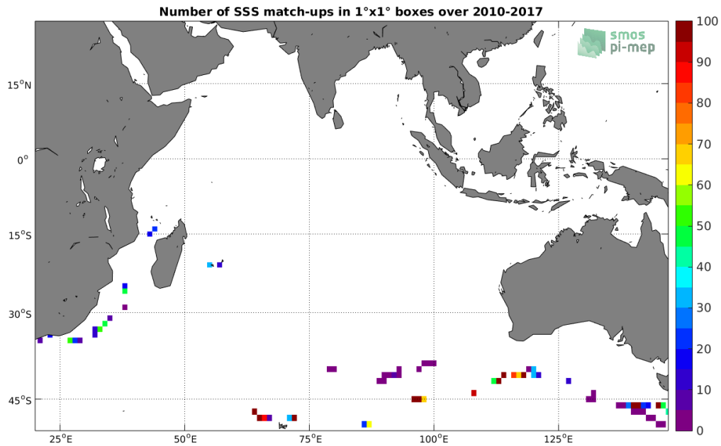
Figure 4: Number of SSS match-ups between TSG-GOSUD-Sailing-ship SSS and the SMOS-L3-CATDS-CPDC-V321-L2Q SSS product for the Indian Ocean Pi-MEP region over 1°x1° boxes and for the full satellite product period.
