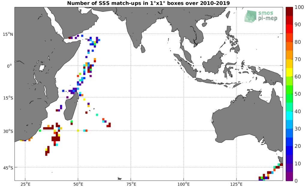
Figure 4: Number of SSS match-ups between TSG (GOSUD-Research-vessel) SSS and the SMOS SSS L2Q v321 - 0.25 Deg (CATDS-CPDC) SSS product for the Indian Ocean Pi-MEP region over 1^\circ \times 1^\circ boxes and for the full satellite product period.
