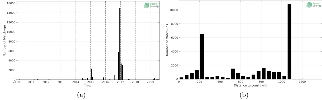
Figure 1: Number of match-ups between TSG (GOSUD-Research-vessel) and SMOS SSS L2Q v321 - 0.25 Deg (CATDS-CPDC) SSS as a function of time (a) and as function of the distance to coast (b) over the Indian Ocean Pi-MEP region and for the full satellite product period.
