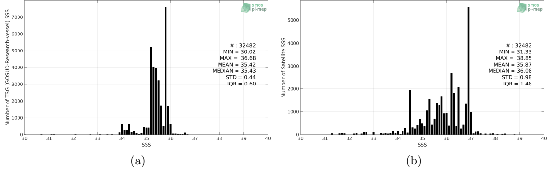
Figure 2: Histograms of SSS from TSG (GOSUD-Research-vessel) (a) and SMOS SSS L2Q v321 - 0.25 Deg (CATDS-CPDC) (b) considering all match-up pairs per bins of 0.1 over the Indian Ocean Pi-MEP region and for the full satellite product period.
