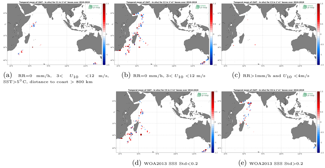
Figure 12: Temporal mean gridded over spatial boxes of size 1^\circ \times 1^\circ of \Delta SSS (SMOS SSS L2Q v321 - 0.25 Deg (CATDS-CPDC) - TSG (GOSUD-Research-vessel)) for 5 different subdatasets corresponding to: RR=0 mm/h, 3 < U_{10} < 12 m/s, SST>5°C, distance to coast > 800 km (a), RR=0 mm/h, 3 < U_{10} < 12 m/s (b), RR>1mm/h and U_{10} < 4 m/s (c), WOA2013 SSS Std<0.2 (d), WOA2013 SSS Std>0.2 (e).
