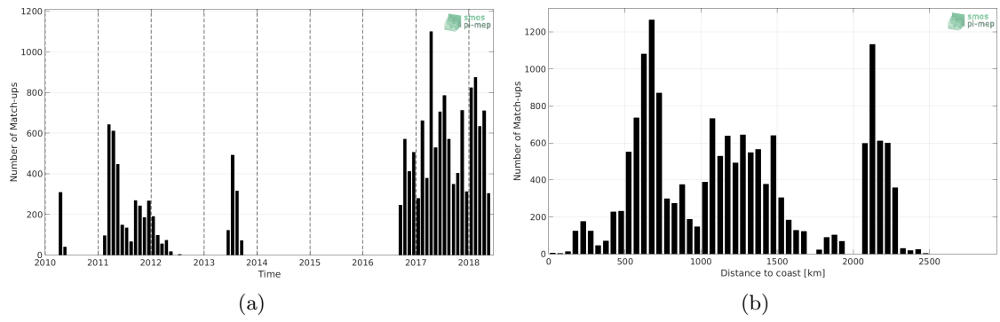
Figure 1: Number of match-ups between Surface drifters and SMOS SSS L2Q v321 - 0.25 Deg (CATDS-CPDC) SSS as a function of time (a) and as function of the distance to coast (b) over the Indian Ocean Pi-MEP region and for the full satellite product period.
