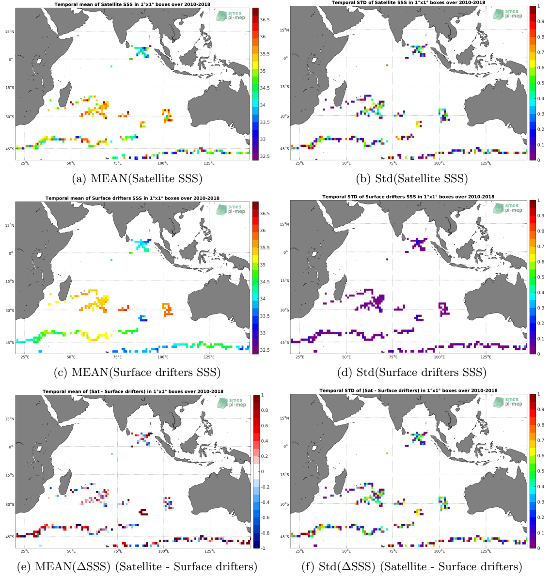
Figure 5: Temporal mean (left) and Std (right) of SSS from SMOS SSS L2Q v321 - 0.25 Deg (CATDS-CPDC) (top), Surface drifters (middle), and of \Delta SSS (Satellite - Surface drifters). Only match-up pairs are used to generate these maps.
