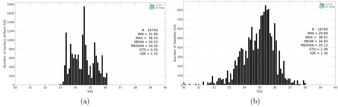
Figure 2: Histograms of SSS from Surface drifters (a) and SMOS SSS L2Q v321 - 0.25 Deg (CATDS-CPDC) (b) considering all match-up pairs per bins of 0.1 over the Indian Ocean Pi-MEP region and for the full satellite product period.
