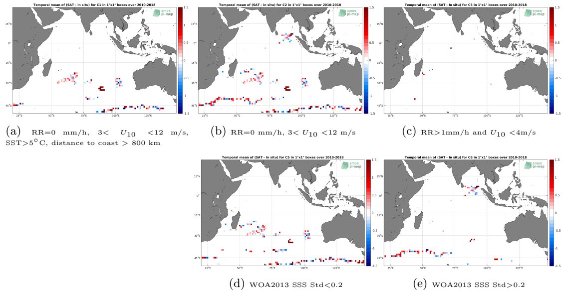
Figure 11: Temporal mean gridded over spatial boxes of size 1^\circ \times 1^\circ of \Delta SSS (SMOS SSS L2Q v321 - 0.25 Deg (CATDS-CPDC) - Surface drifters) for 5 different subdatasets corresponding to: RR=0 mm/h, 3 < U_{10} < 12 m/s, SST > 5^\circ\text{C} , distance to coast > 800 km (a), RR=0 mm/h, 3 < U_{10} < 12 m/s (b), RR > 1 mm/h and U_{10} < 4 m/s (c), WOA2013 SSS Std < 0.2 (d), WOA2013 SSS Std > 0.2 (e).
