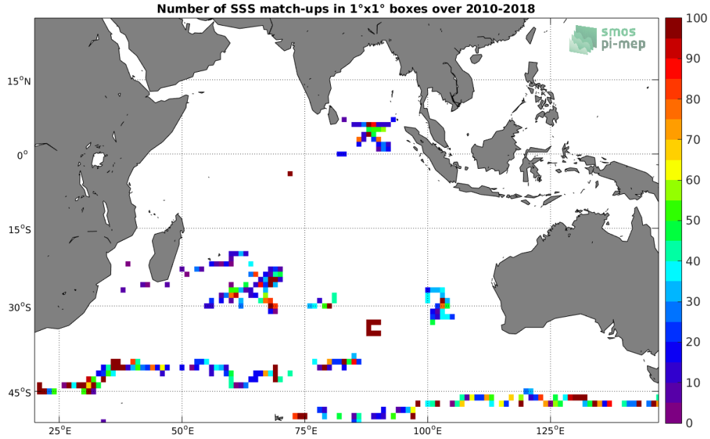
Figure 3: Number of SSS match-ups between Surface drifters SSS and the SMOS SSS L2Q v321 - 0.25 Deg (CATDS-CPDC) SSS product for the Indian Ocean Pi-MEP region over 1^\circ \times 1^\circ boxes and for the full satellite product period.
