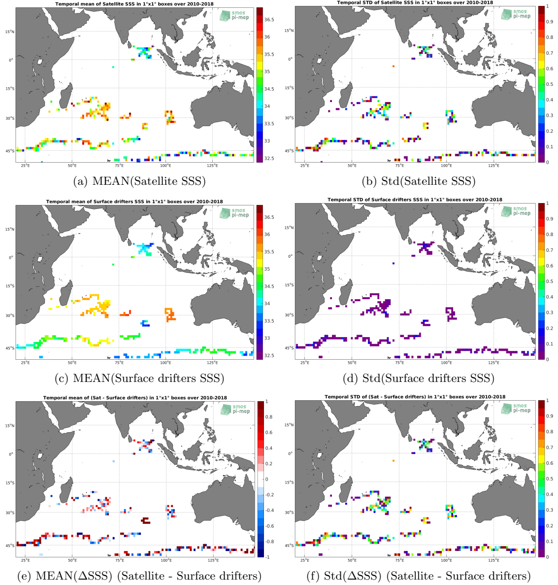
Figure 5: Temporal mean (left) and Std (right) of SSS from SMOS L2Q v321 - 0.25 Deg (CATDS-CPDC) (top), Surface drifters (middle), and of \Delta SSS (Satellite - Surface drifters). Only match-up pairs are used to generate these maps.
