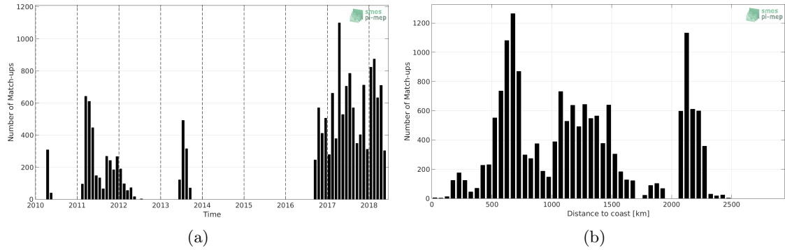
Figure 1: Number of match-ups between Surface drifters and SMOS L2Q v321 - 0.25 Deg (CATDS-CPDC) SSS as a function of time (a) and as function of the distance to coast (b) over the Indian Ocean Pi-MEP region and for the full satellite product period.
