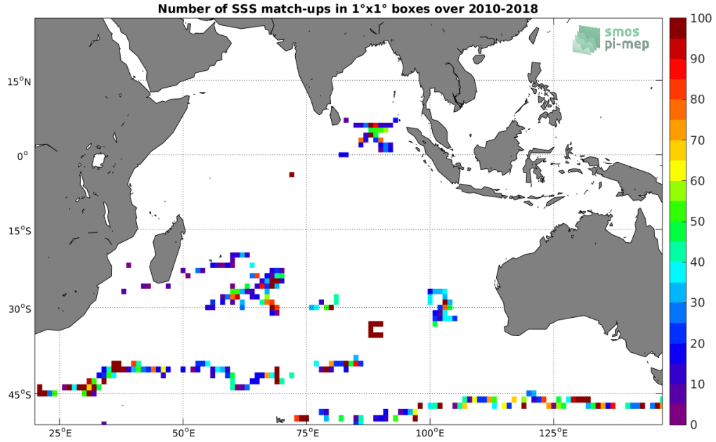
Figure 3: Number of SSS match-ups between Surface drifters SSS and the SMOS L2Q v321 - 0.25 Deg (CATDS-CPDC) SSS product for the Indian Ocean Pi-MEP region over 1^\circ \times 1^\circ boxes and for the full satellite product period.
