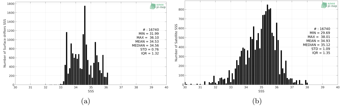
Figure 2: Histograms of SSS from Surface drifters (a) and SMOS L2Q v321 - 0.25 Deg (CATDS-CPDC) (b) considering all match-up pairs per bins of 0.1 over the Indian Ocean Pi-MEP region and for the full satellite product period.
