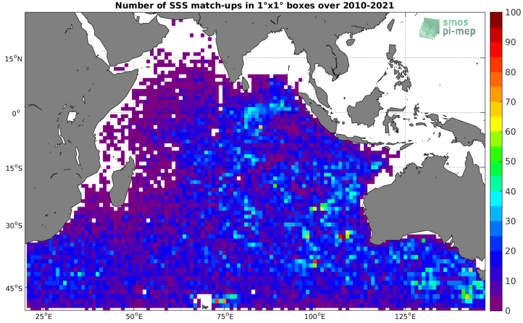
Figure 4: Number of SSS match-ups between Argo SSS and the SMOS SSS L2Q v321 - 0.25 Deg (CATDS-CPDC) SSS product for the Indian Ocean Pi-MEP region over 1^\circ \times 1^\circ boxes and for the full satellite product period.
