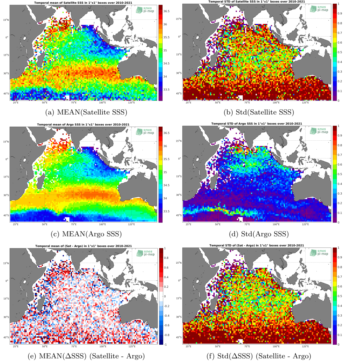
Figure 6: Temporal mean (left) and Std (right) of SSS from SMOS SSS L2Q v321 - 0.25 Deg (CATDS-CPDC) (top), Argo (middle), and of \Delta SSS (Satellite - Argo). Only match-up pairs are used to generate these maps.
