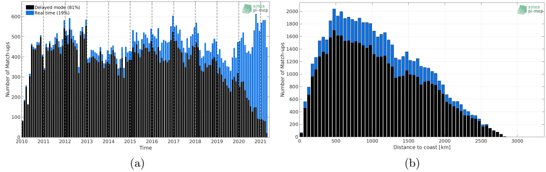
Figure 1: Number of match-ups between Argo and SMOS SSS L2Q v321 - 0.25 Deg (CATDS-CPDC) SSS as a function of time (a) and as function of the distance to coast (b) over the Indian Ocean Pi-MEP region and for the full satellite product period.
