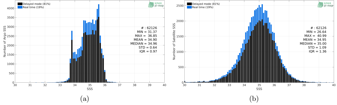
Figure 2: Histograms of SSS from Argo (a) and SMOS SSS L2Q v321 - 0.25 Deg (CATDS-CPDC) (b) considering all match-up pairs per bins of 0.1 over the Indian Ocean Pi-MEP region and for the full satellite product period.
